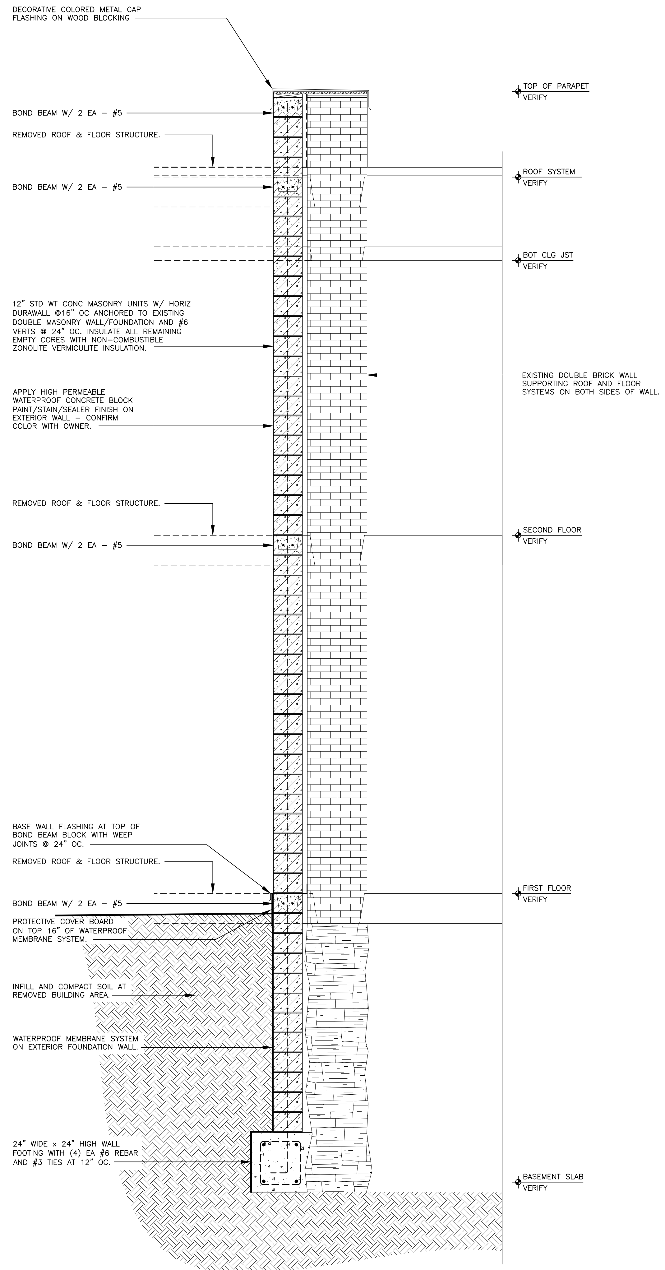
1 WALL SECTION 1/2" = 1'-0"
