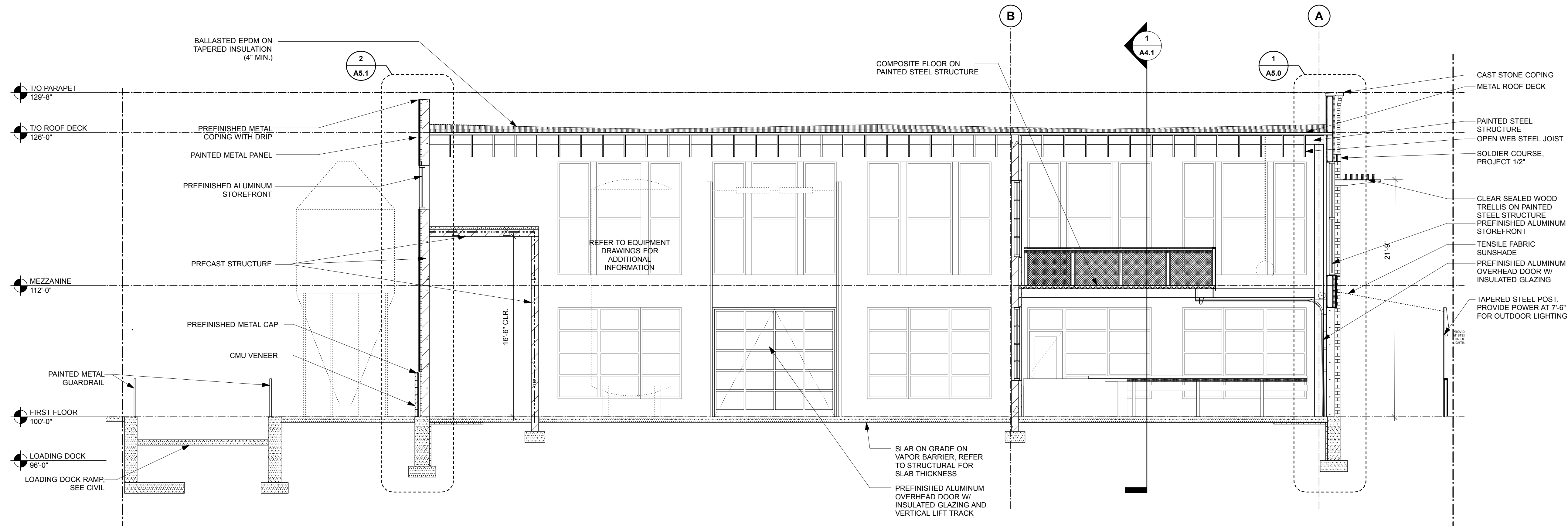
2 A4.0 BUILDING SECTION SCALE: 3/16" = 1'-0"
