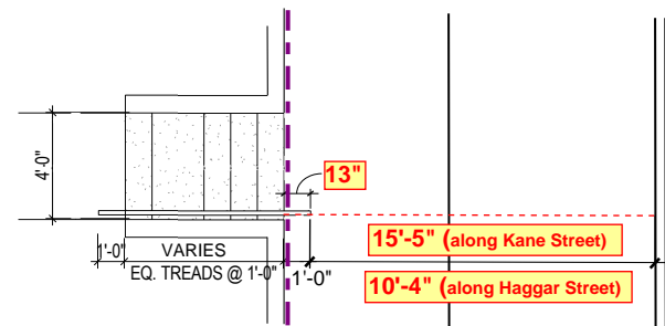
TYPICAL WALK UP UNIT STAIRS
