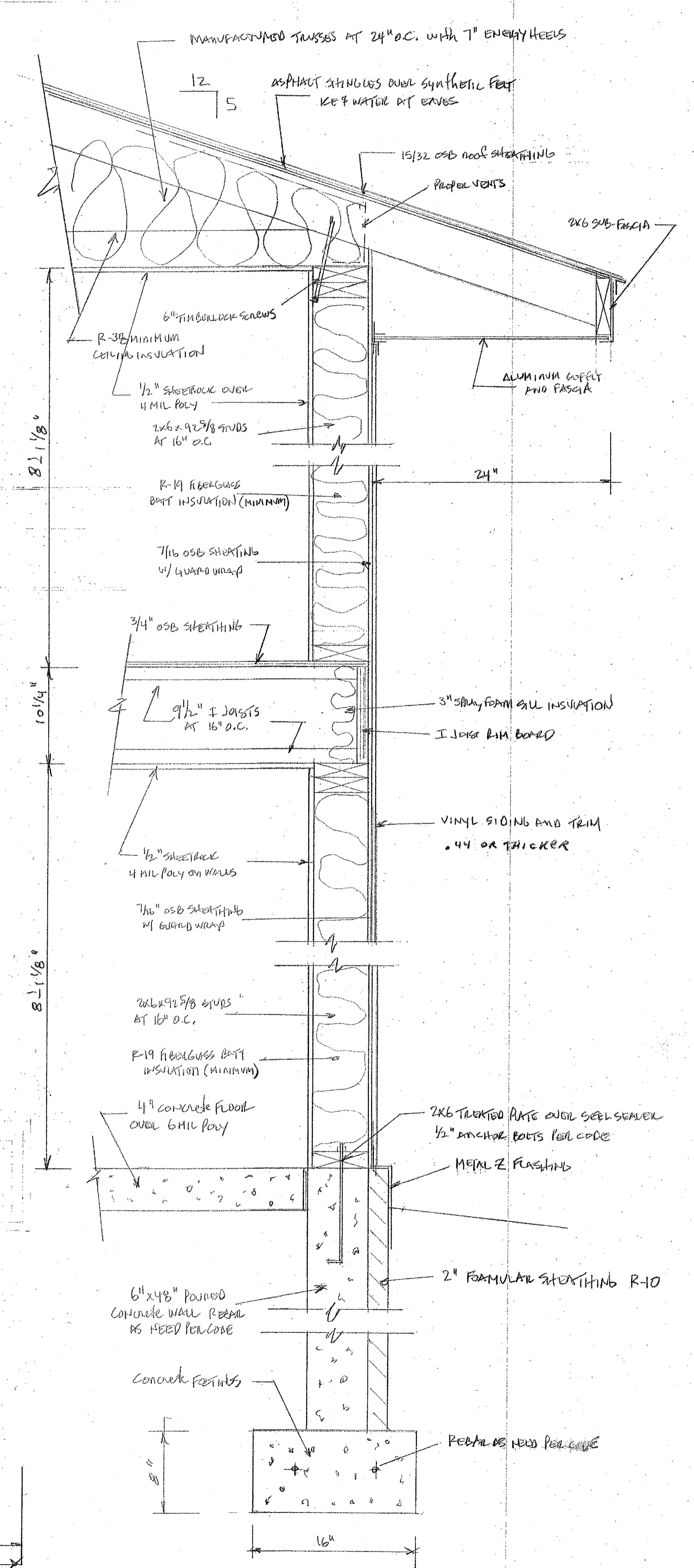
Cross Section 3/4" = 1'-0"
