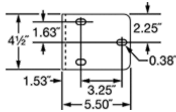
Mounting Bracket
