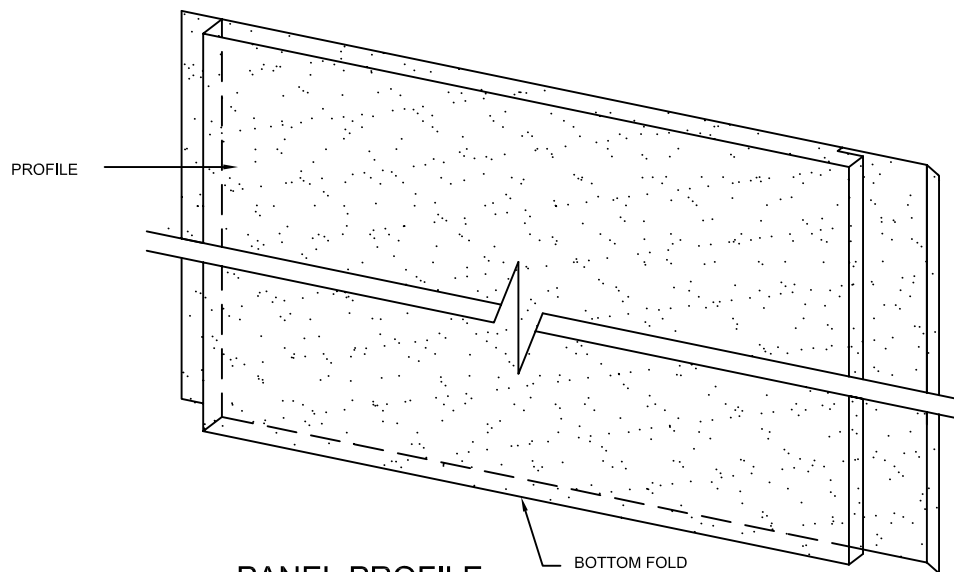
PANEL PROFILE
