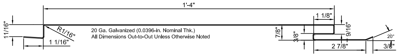
PLAN VIEW
