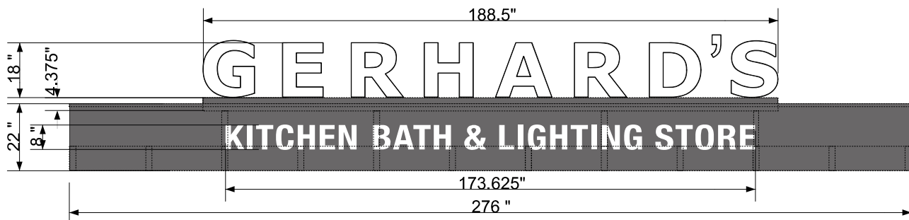
AWNING FRONT VIEW WITH FACE
