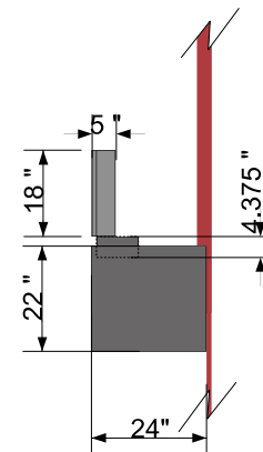
ENLARGED SIDE VIEW W/O END SKIN
