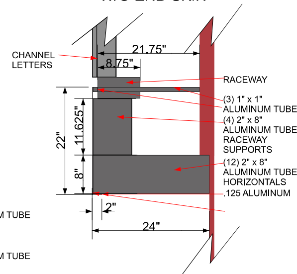
ENLARGED SIDE VIEW W/O END SKIN
