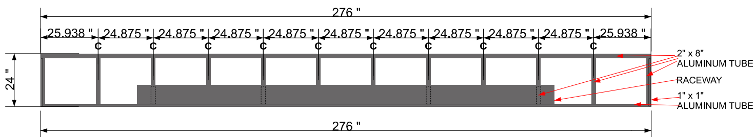
AWNING TOP VIEW
