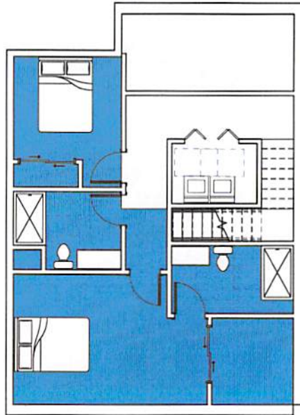
2 2nd Level, TYP SCALE: 1/8" = 1'-0"
