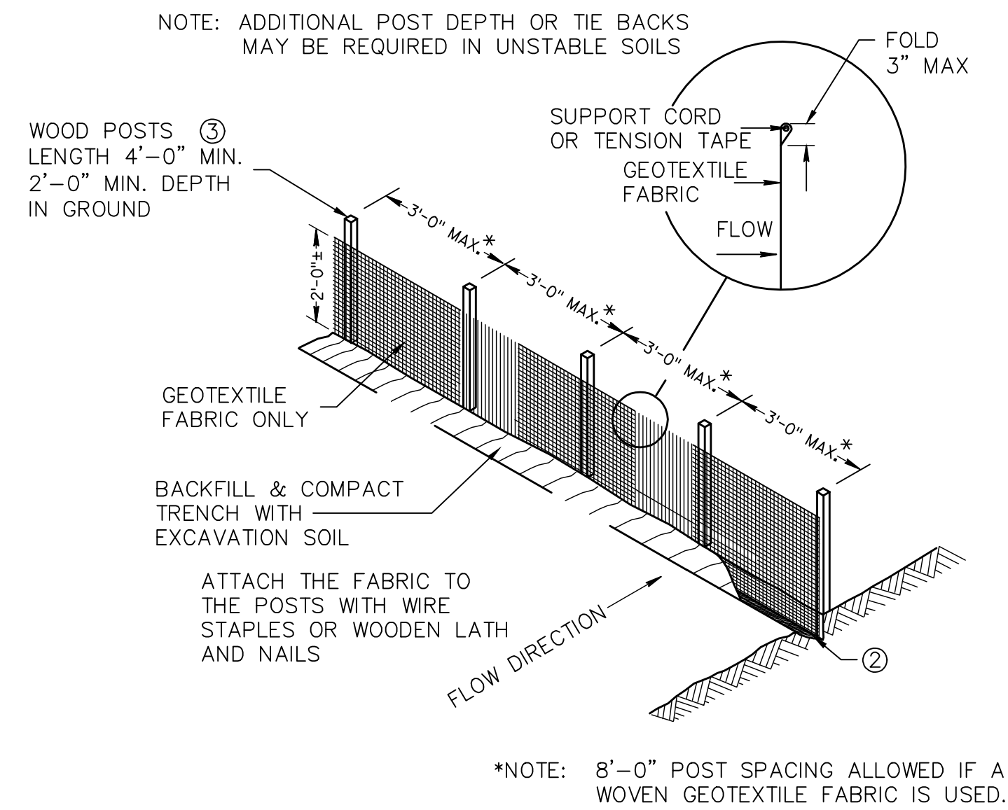
SILT FENCE
