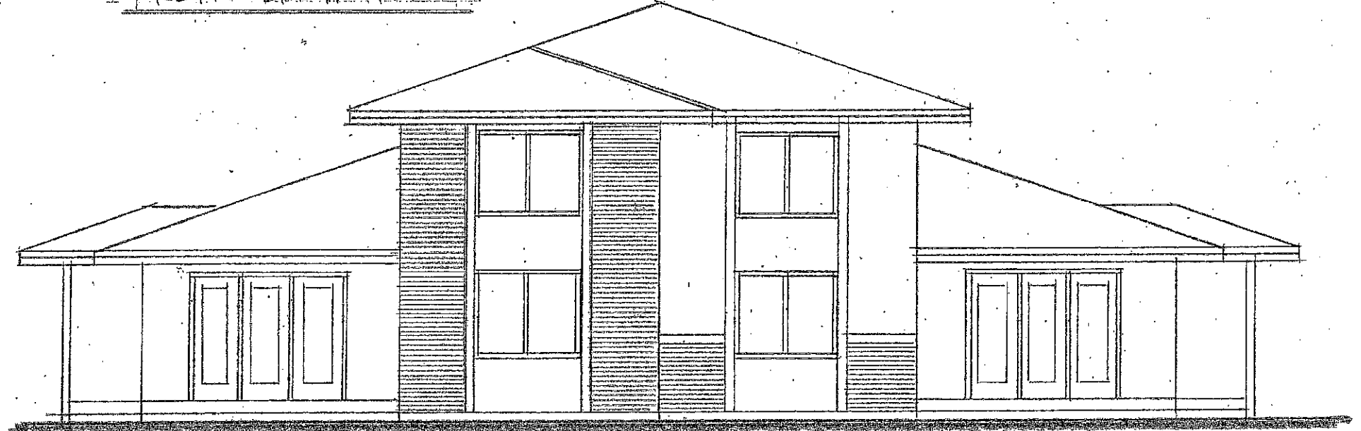
REAR ELEVATION
