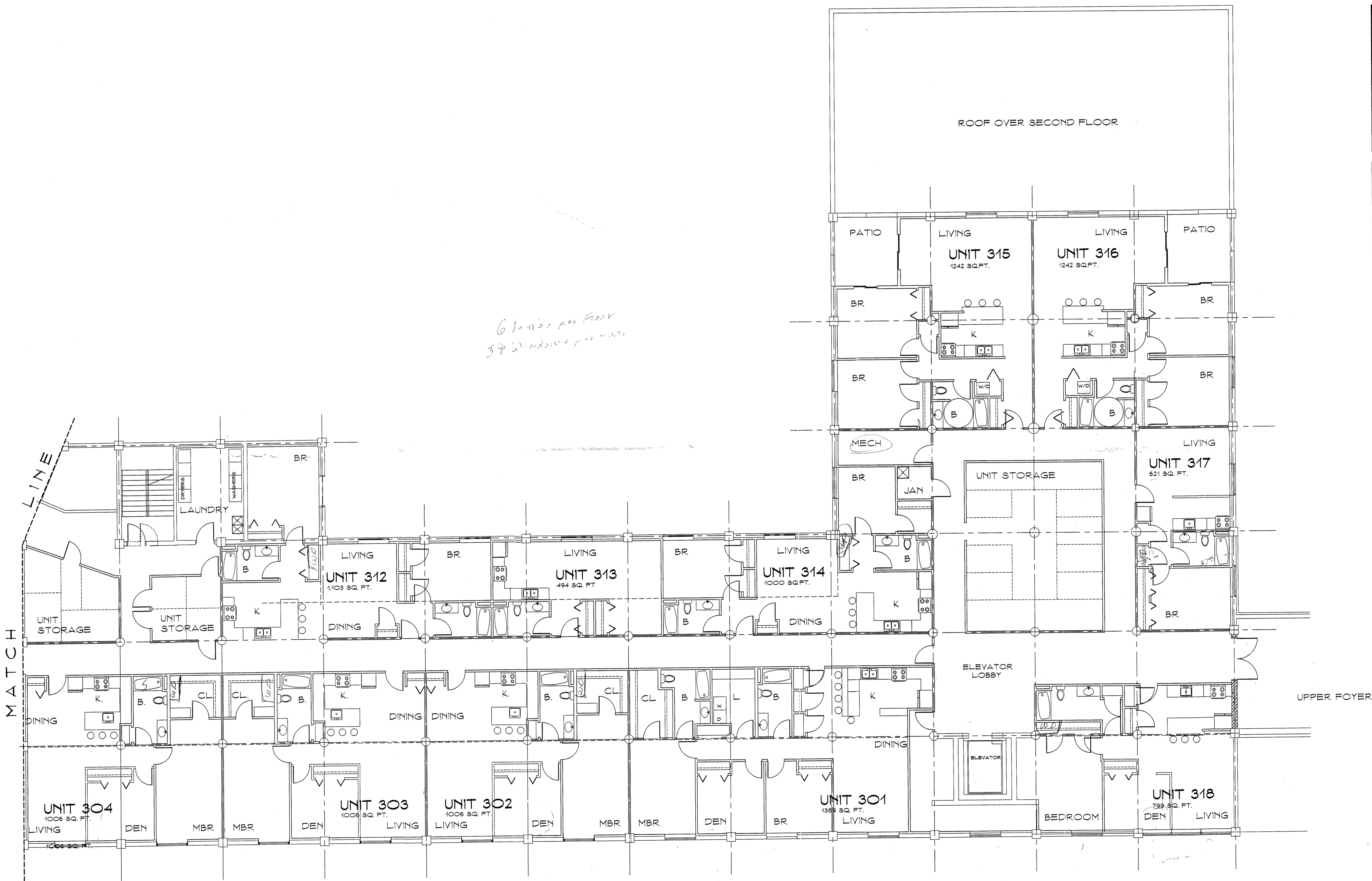
PARTIAL THIRD FLOOR PLAN SCALE 1/8" = 1'-0"
