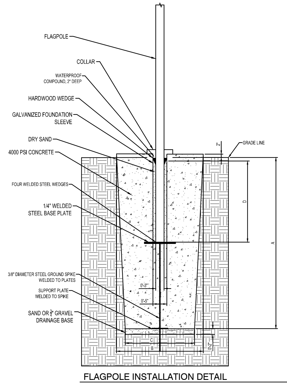
FLAGPOLE INSTALLATION DETAIL NTS
