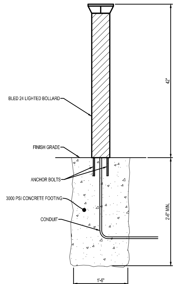
LIGHTED BOLLARD NTS
