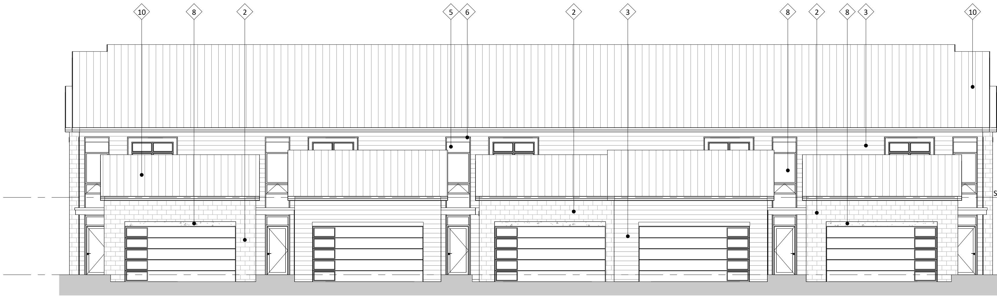
1 ELEVATION - NORTH A201 1/8" = 1'-0"
