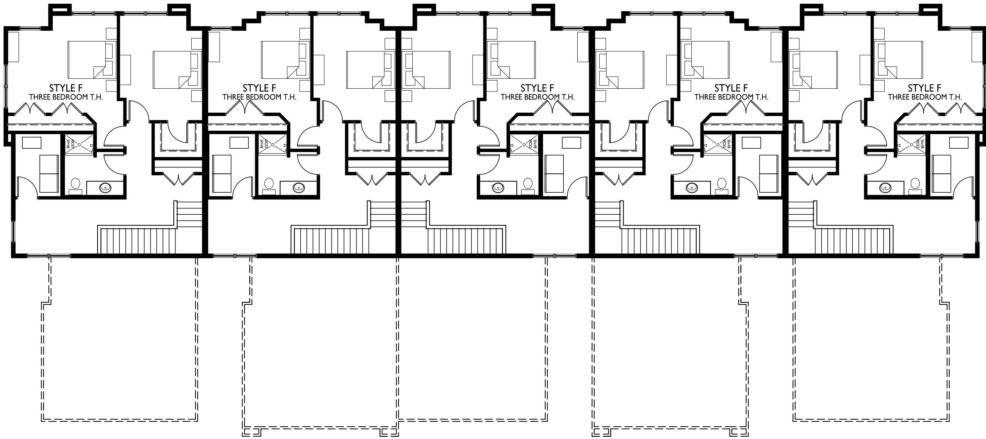
2 A102 1/8" = 1'-0" 5-UNIT TOWNHOUSE SECOND FLOOR
