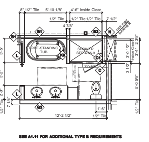
SEE A1.11 FOR ADDITIONAL TYPE B REQUIREMENTS
