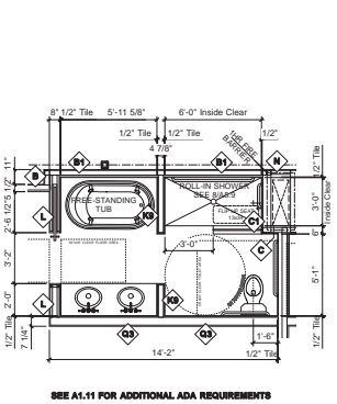
SEE A1.11 FOR ADDITIONAL ADA REQUIREMENTS
