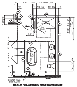
SEE A1.11 FOR ADDITIONAL TYPE B REQUIREMENTS
