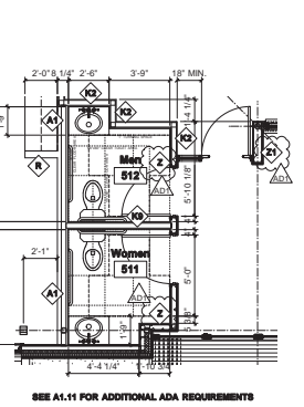
SEE A1.11 FOR ADDITIONAL ADA REQUIREMENTS
