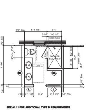
SEE A1.11 FOR ADDITIONAL TYPE B REQUIREMENTS
