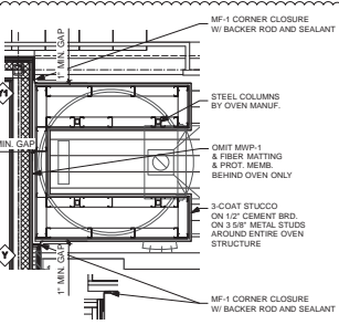
8 PIZZA OVEN PLAN SCALE: 1/2" = 1'-0"
