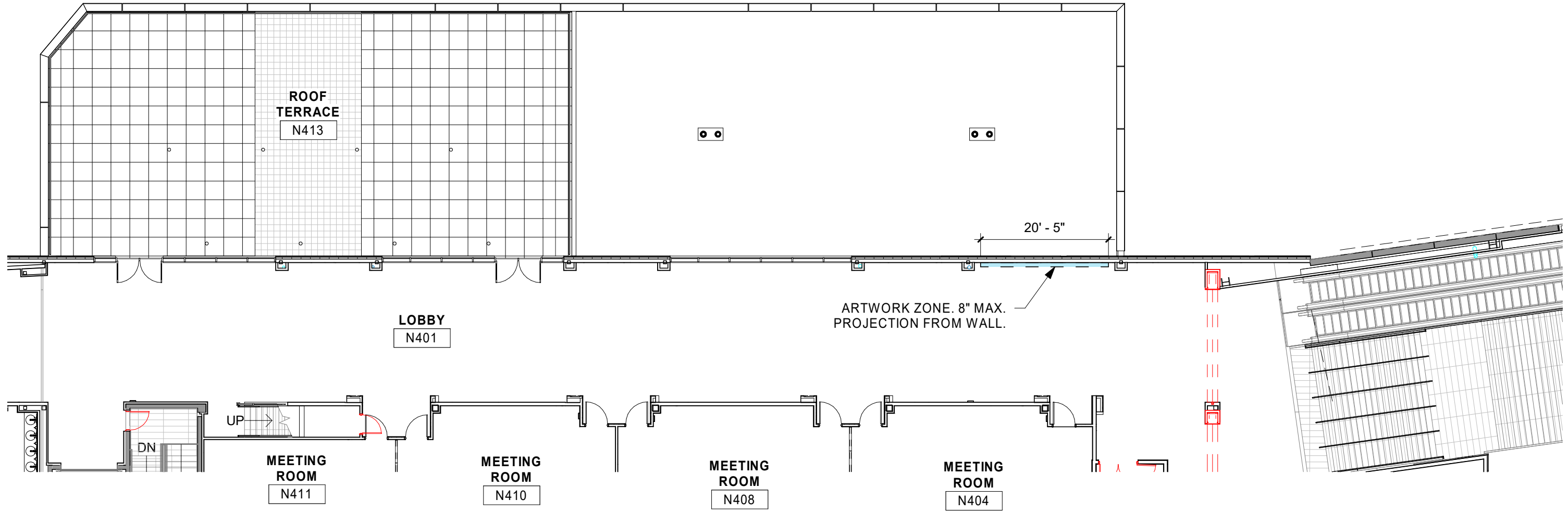
1 BALLROOM LEVEL PARTIAL FLOOR PLAN 1/16" = 1'-0"
