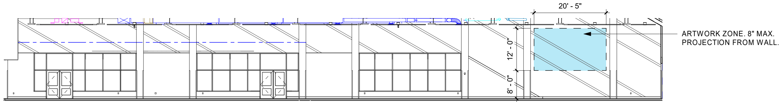
2 LOBBY N401 - NORTH ARTWORK 1/16" = 1'-0"
