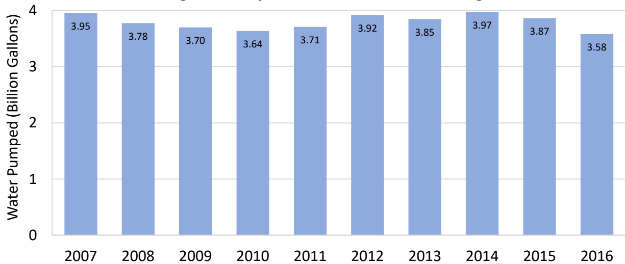
Figure 28: City of La Crosse Annual Water Usage
