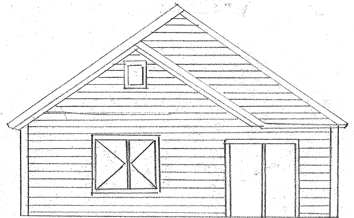
BACK ELEVATION
