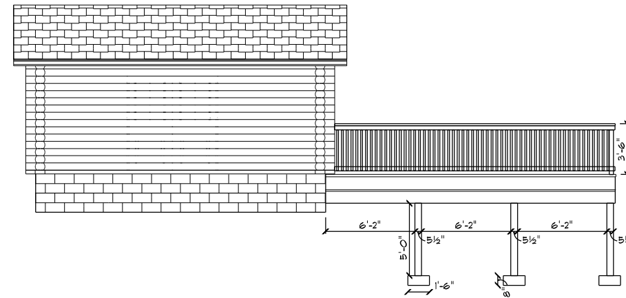
East Elevation
