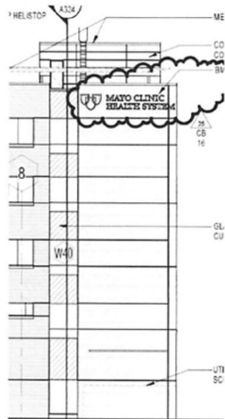
South Elevation
