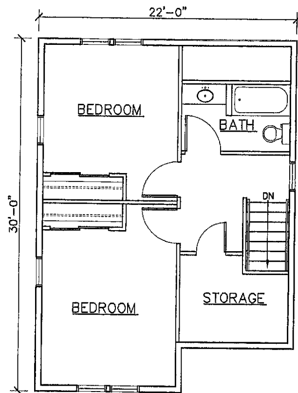
2 A5 SECOND FLOOR PLAN 624 S.F. 1/8" = 1'-0"
