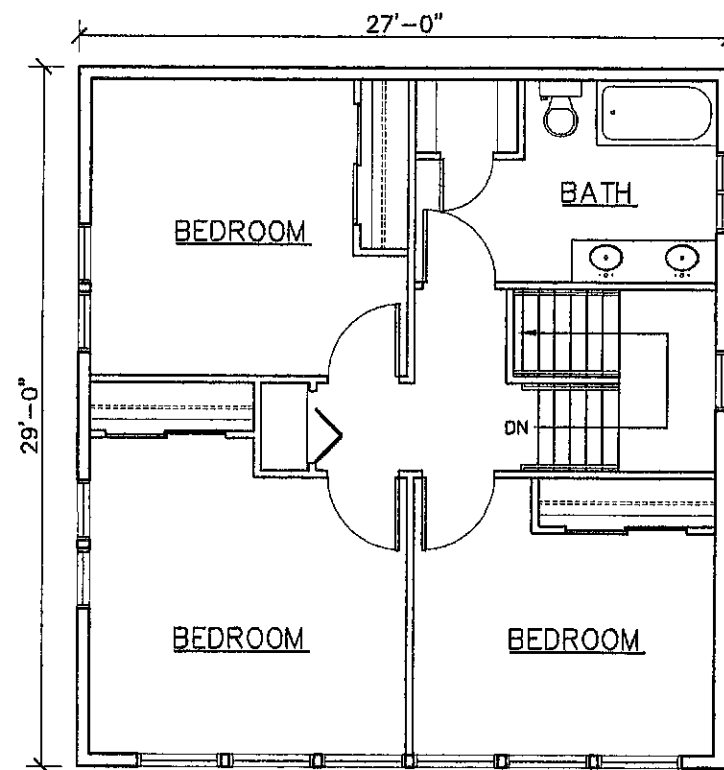
2 SECOND FLOOR PLAN 783 S.F. A4 1/8" = 1'-0"
