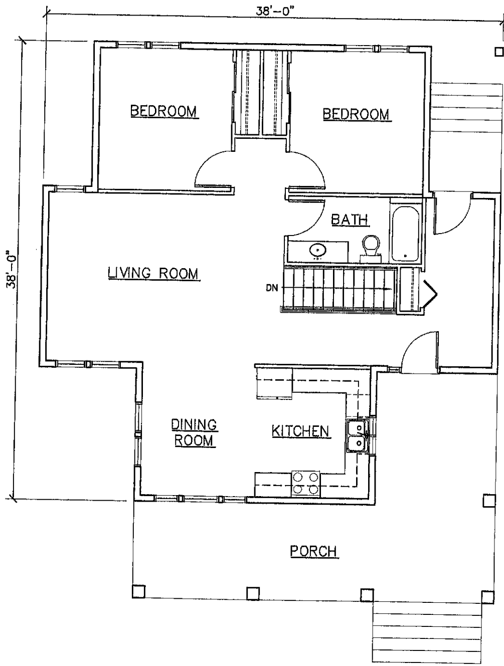
1 A2 FLOOR PLAN 1,126 S.F. 1/8" = 1'-0"
