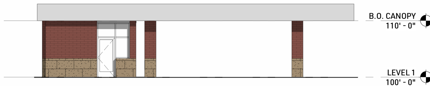
2 CASHIER BUILDING - NORTH EXTERIOR COLOR 3/32" = 1'-0"
