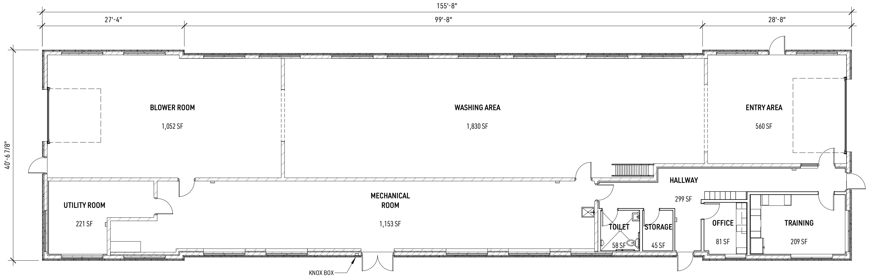
1 FLOOR PLAN 3/32" = 1'-0"
