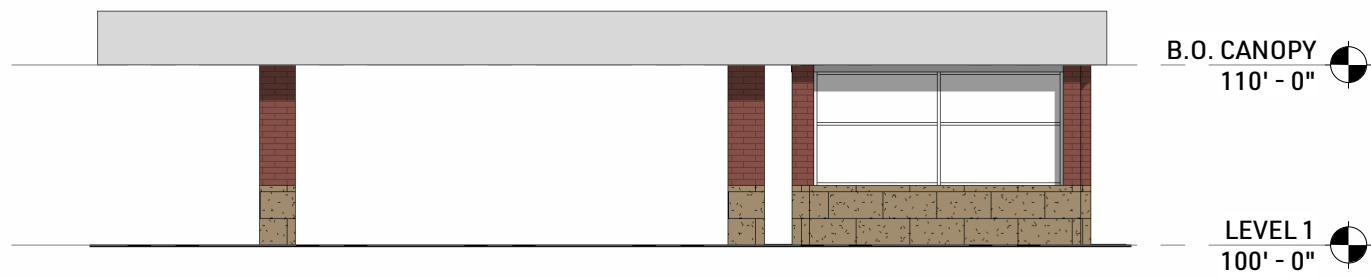
4 CASHIER BUILDING - SOUTH EXTERIOR COLOR 3/32" = 1'-0"
