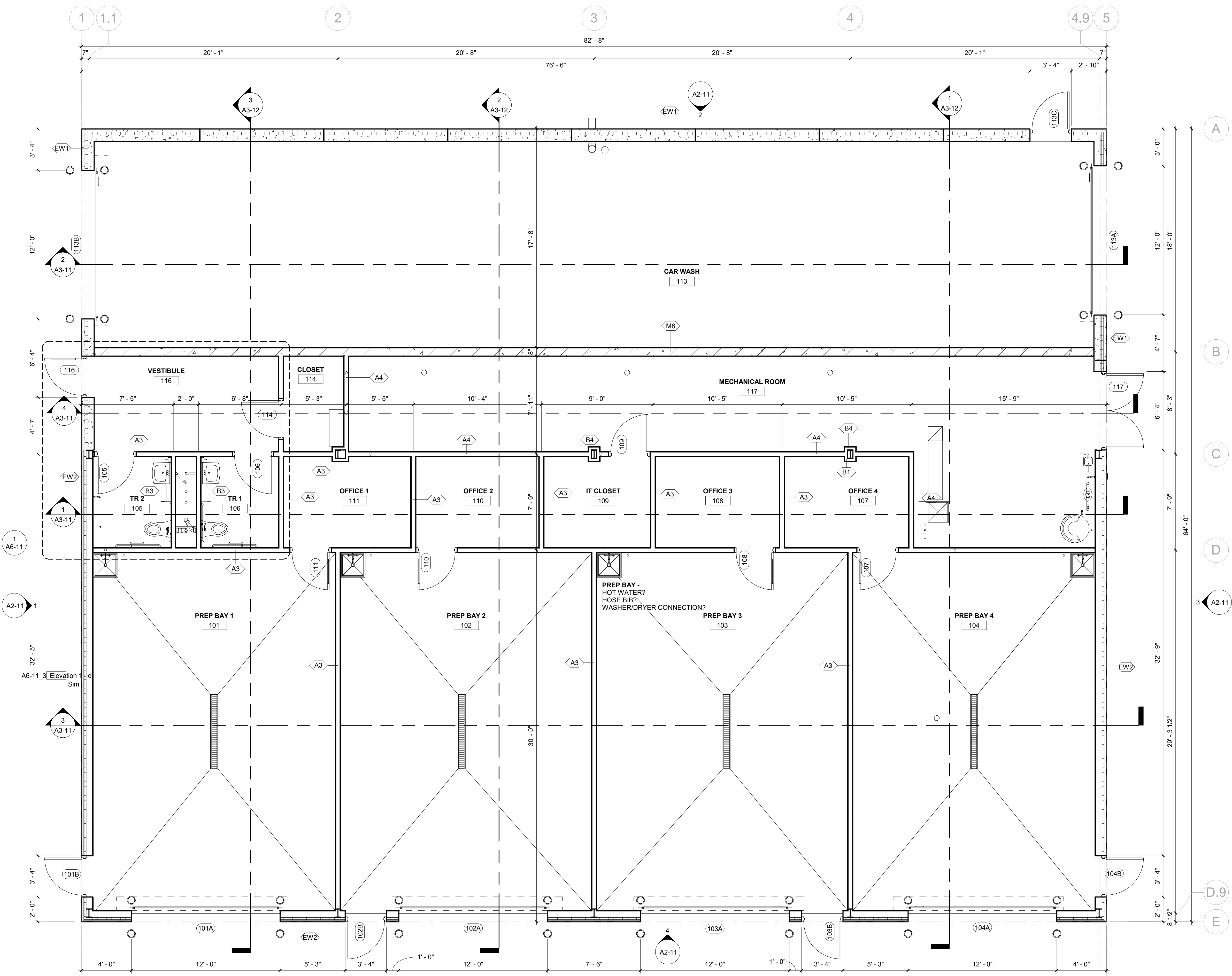
1 FLOOR PLAN 1/4" = 1'-0"
