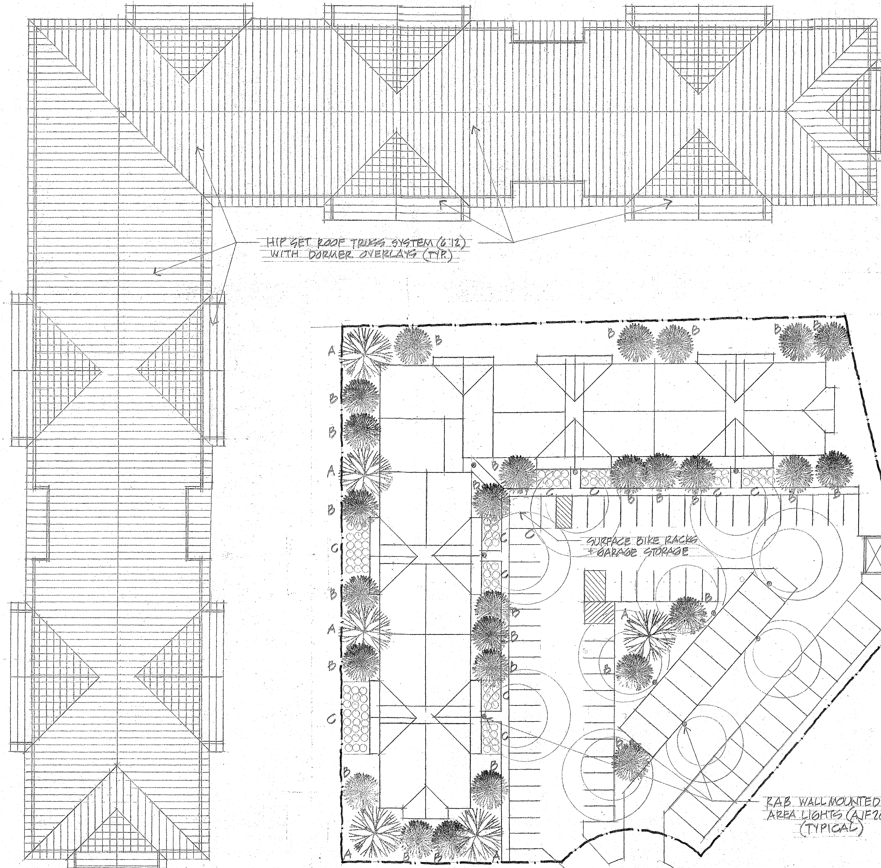
ROOF FRAMING PLAN 1"=100'
