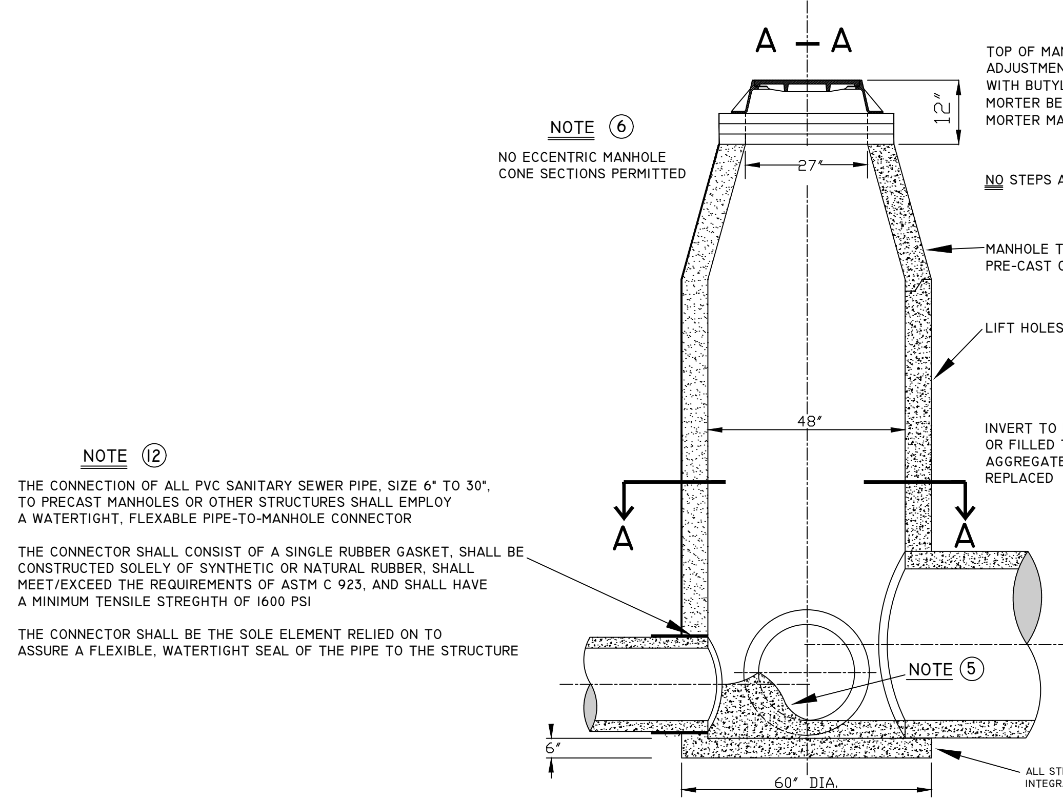
C D-6 DETAILS OF STANDARD MANHOLE FOR 30" PIPE OR SMALLER
