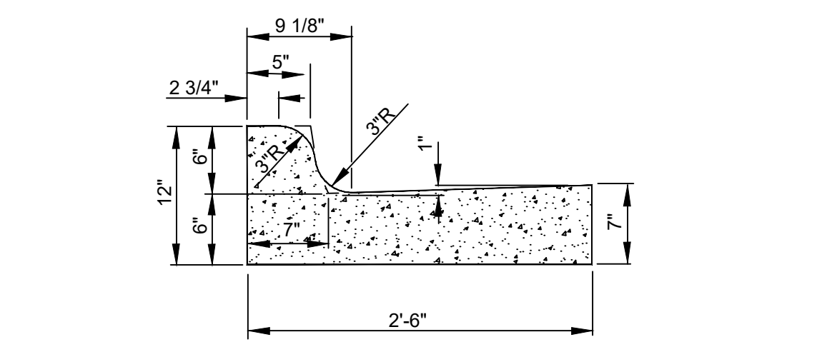
STANDARD CURB & GUTTER SECTION
