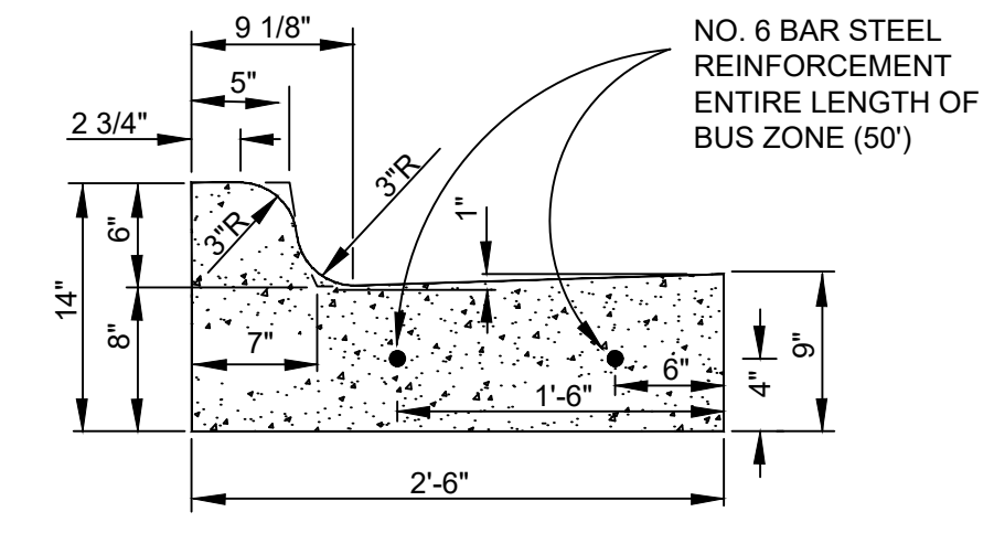
REINFORCED CURB & GUTTER SECTION (BUS STOP LOCATIONS)
