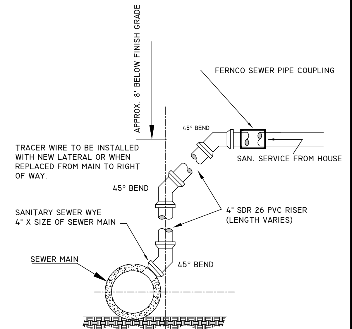
DETAILS OF RISER FOR HOUSE CONNECTION
