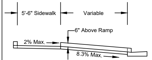
Section Y-Y (PED Curb tied if adjacent to TURF)
