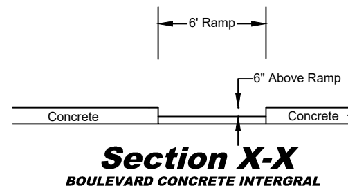
Section X-X BOULEVARD CONCRETE NON-INTERGRAL
