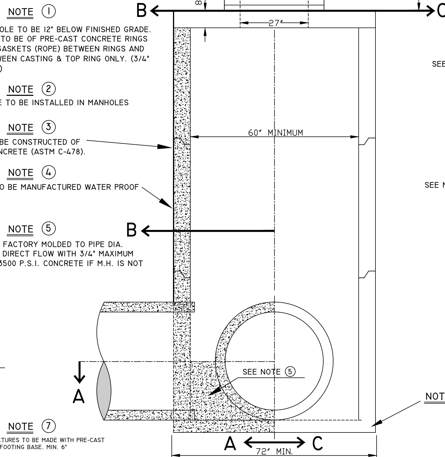
D D-6 DETAILS OF STANDARD MANHOLE FOR 36" PIPE OR LARGER
