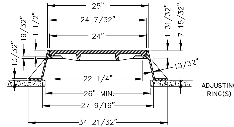
A - A DETAIL OF MANHOLE FRAME & COVER
