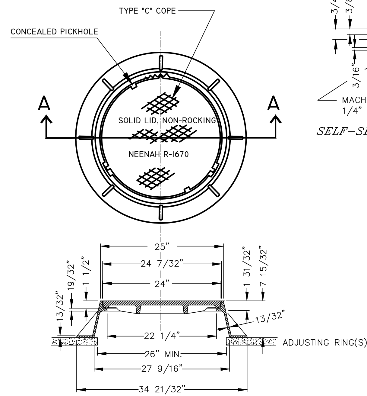
DETAIL OF MANHOLE FRAME & COVER
