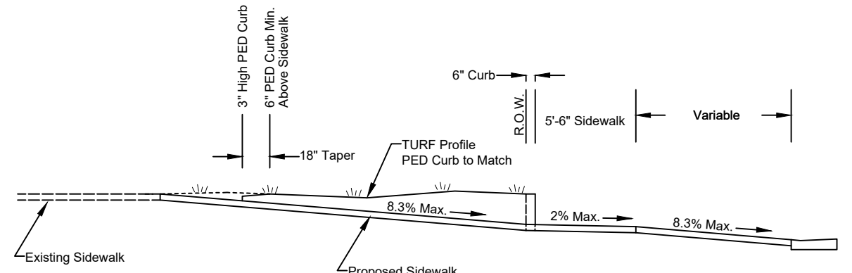
Section Z-Z Turf
