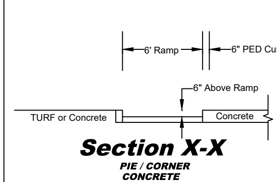
Section X-X PIE / CORNER TURF
