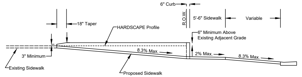
Section Z-Z Hardscape
