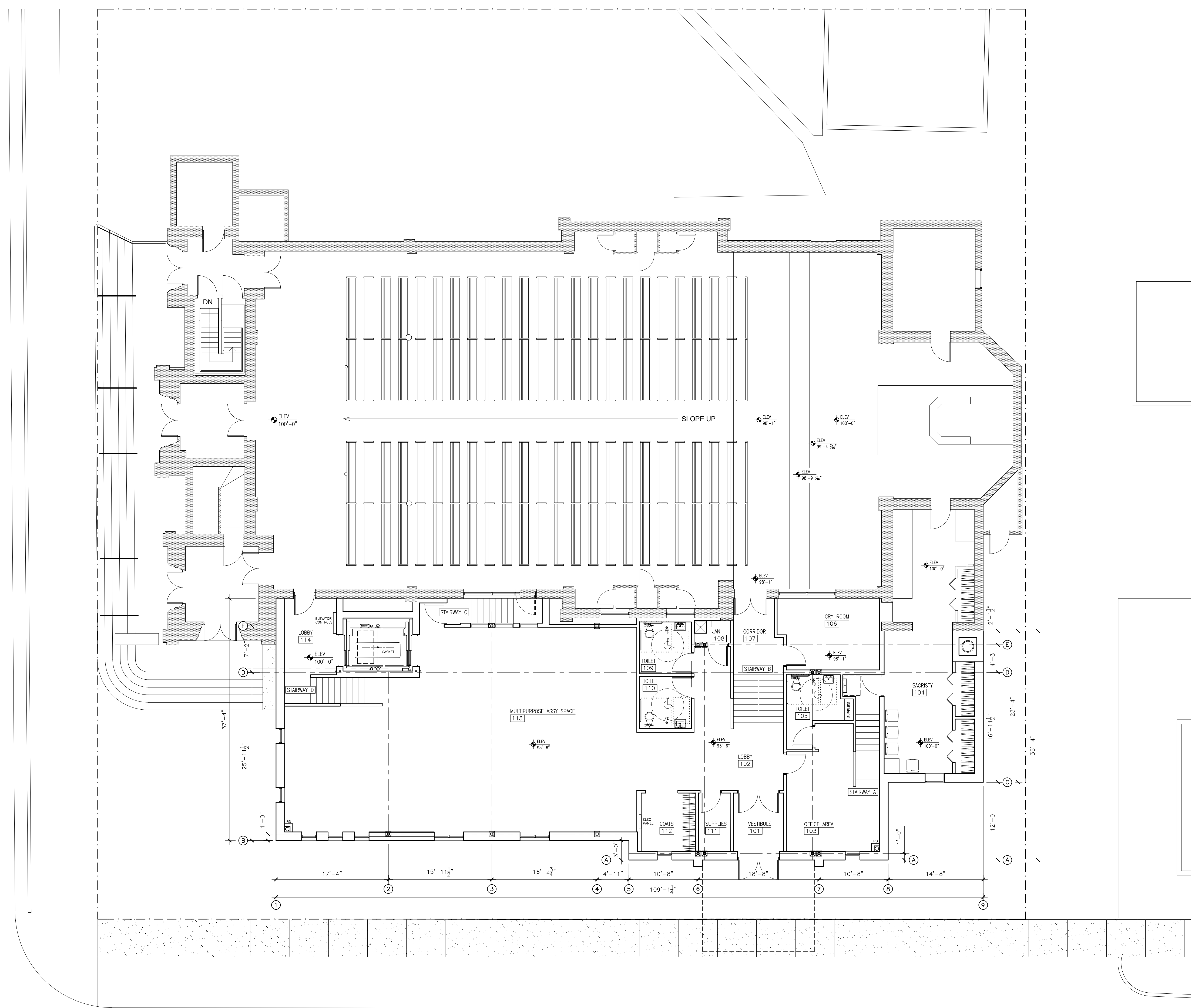
1 EXISTING & ADDITION FIRST FLOOR PLAN 1/8" = 1'-0"
