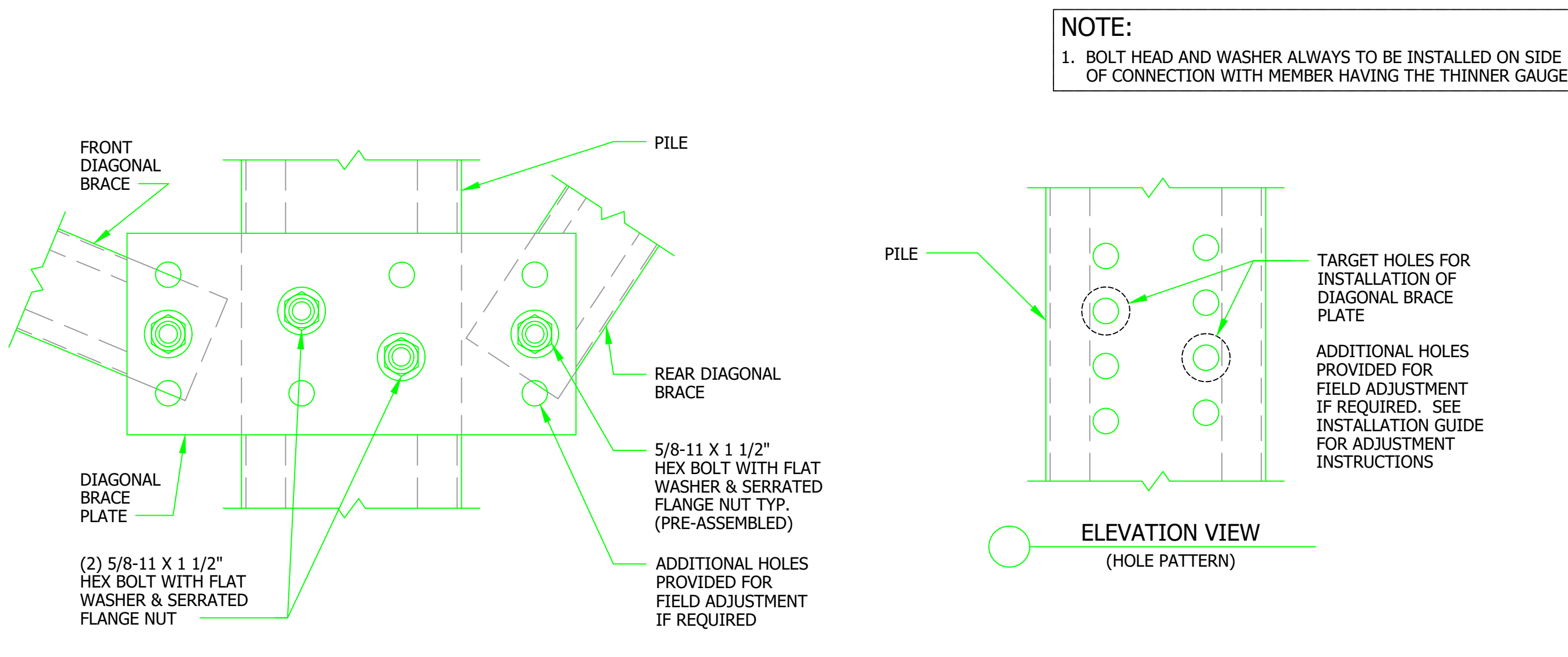
507 DIAGONAL BRACE TO PILE CONNECTION
