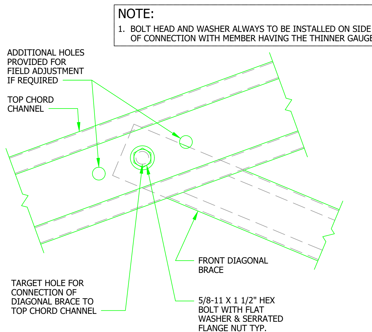
505 TOP CHORD TO DIAGONAL BRACE CONNECTION (FRONT BRACE)
