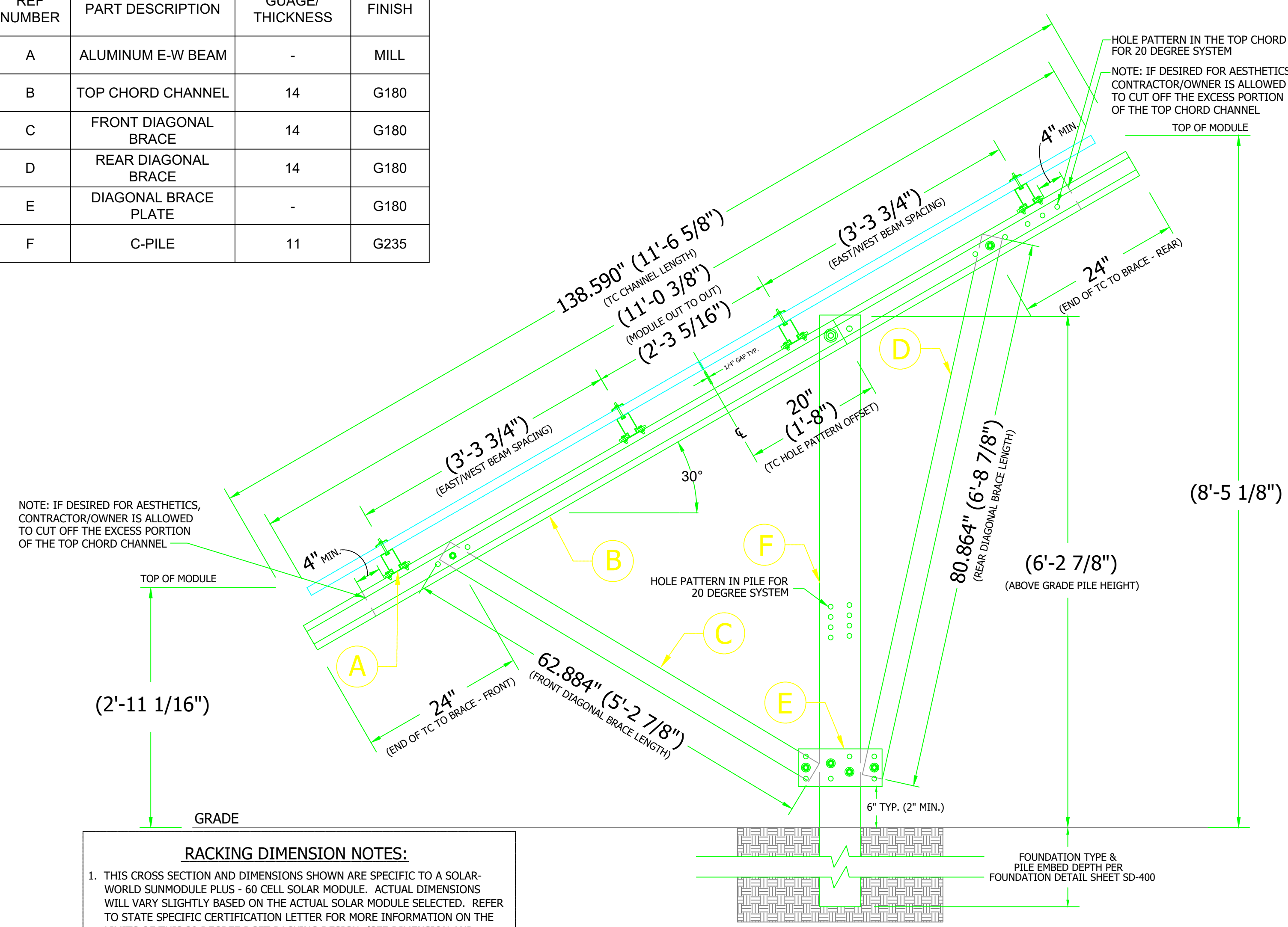
SECTION VIEW OF TABLE (60 CELL SOLAR PANELS) (30 DEGREE TILT)
