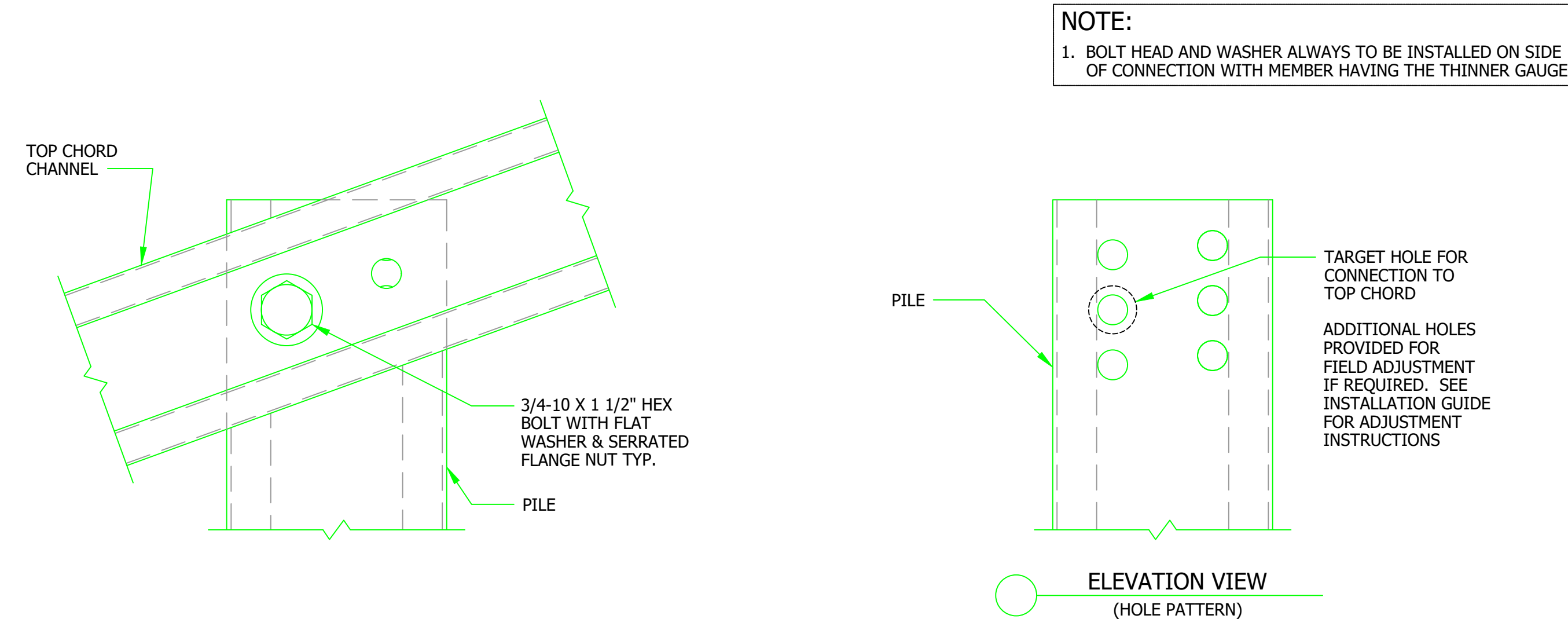
504 TOP CHORD TO PILE CONNECTION
