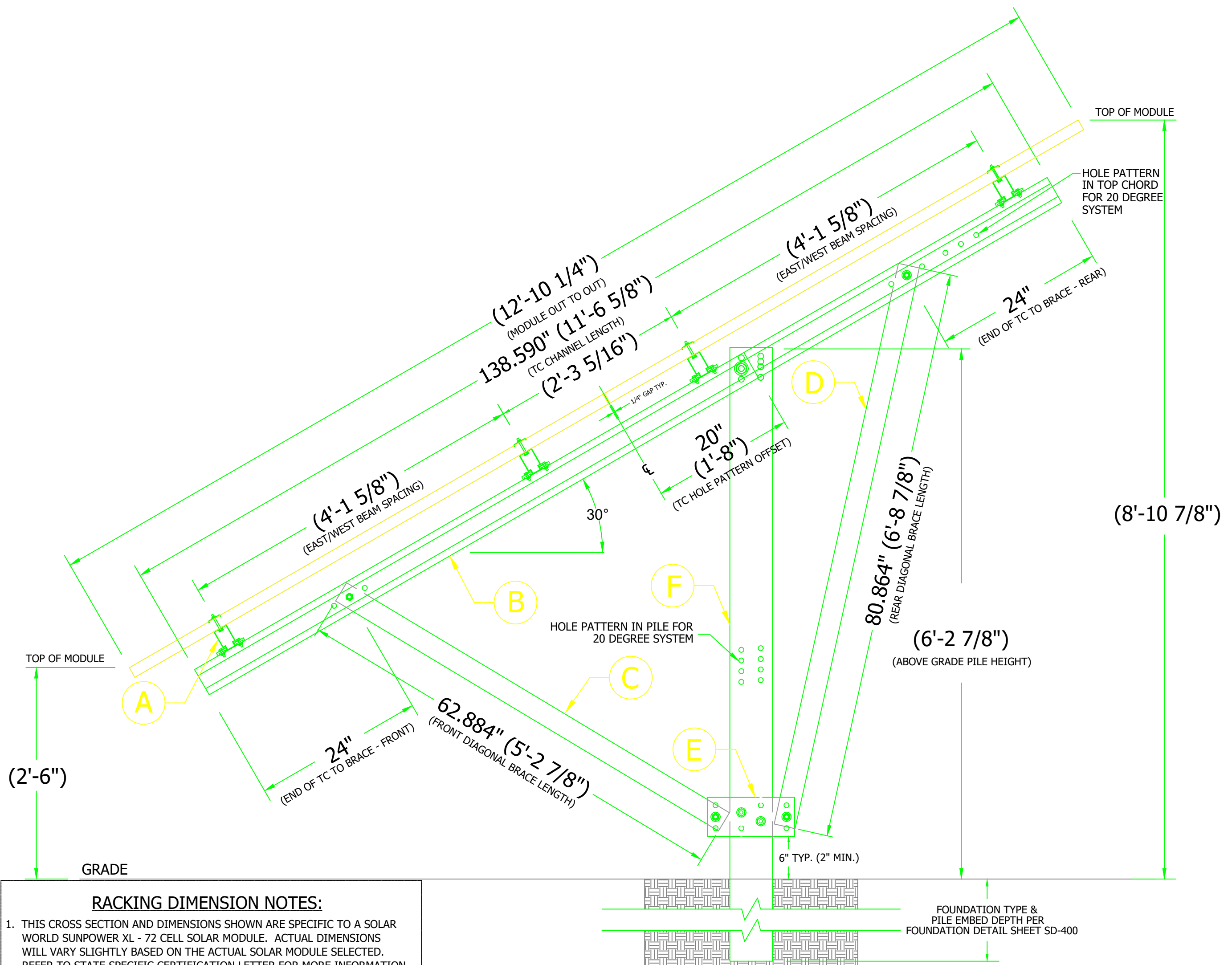
SECTION VIEW OF TABLE (72 CELL SOLAR PANELS) (30 DEGREE TILT)
