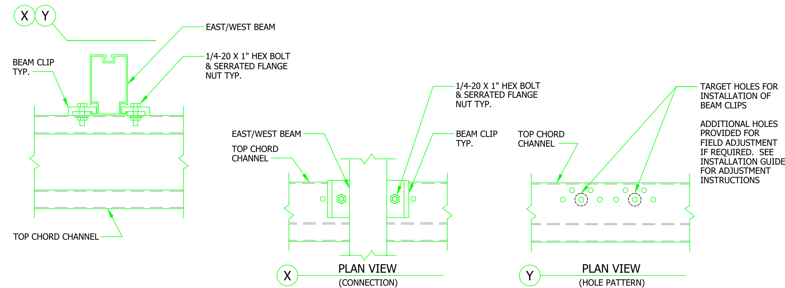
503 EAST/WEST BEAM TO TOP CHORD CONNECTION
