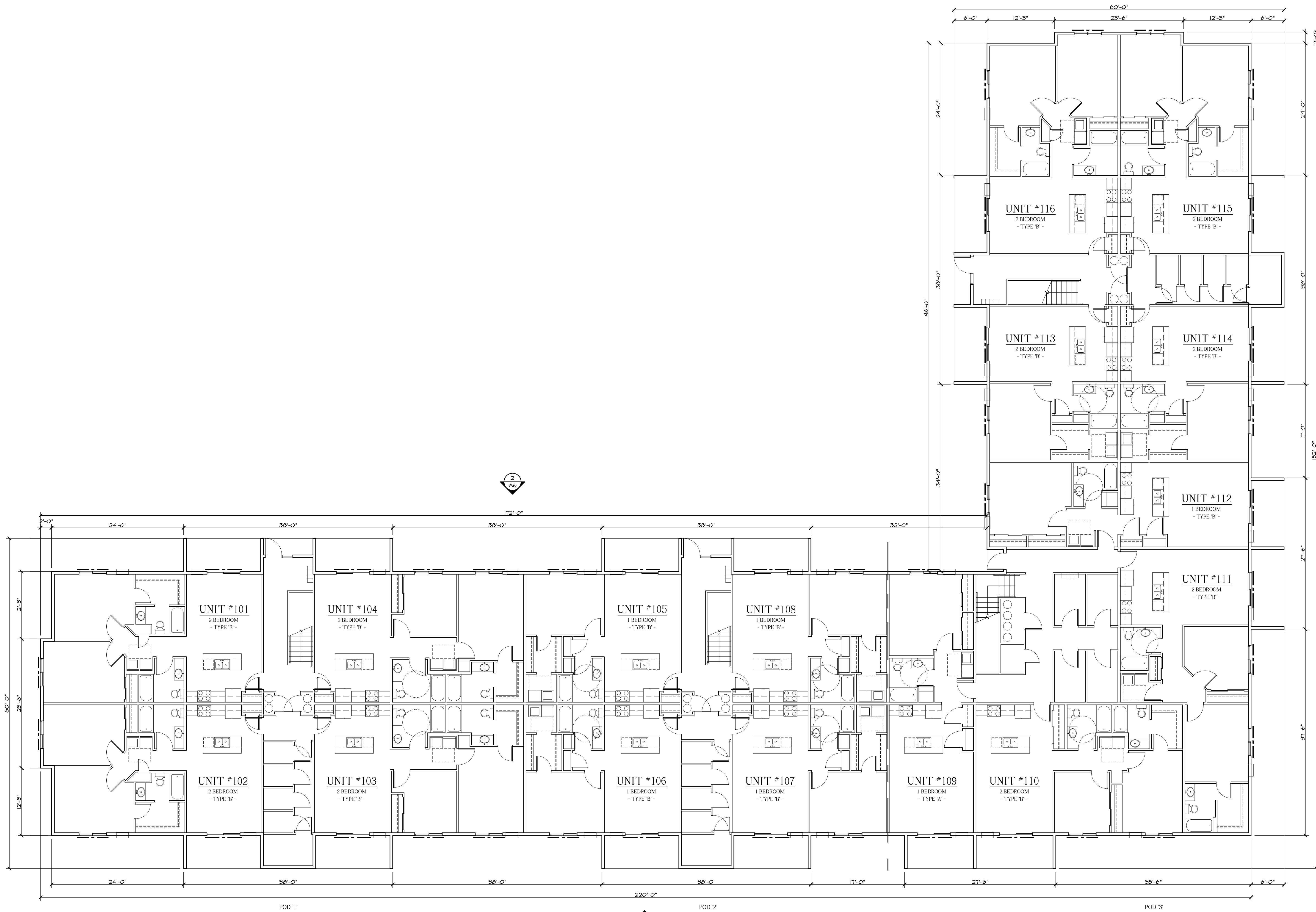
1 AI FIRST FLOOR PLAN 1/8" = 1'-0"
