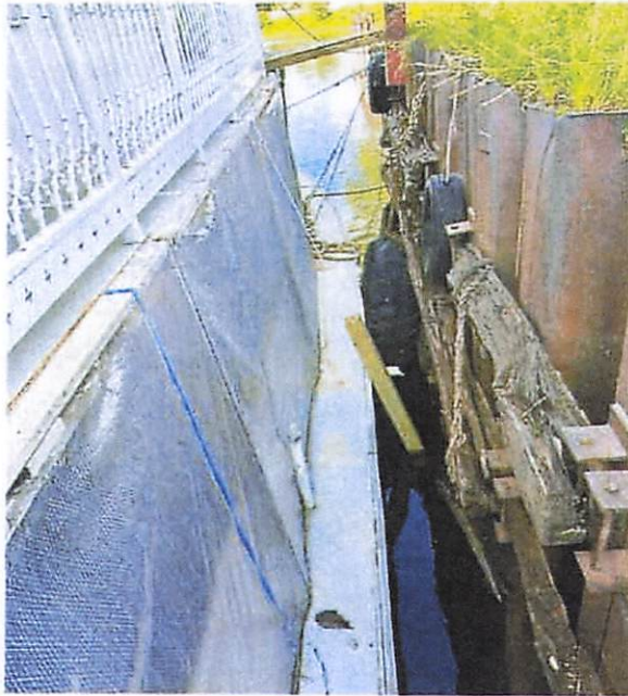
Figure 5: Sheet Pile Wall Front
