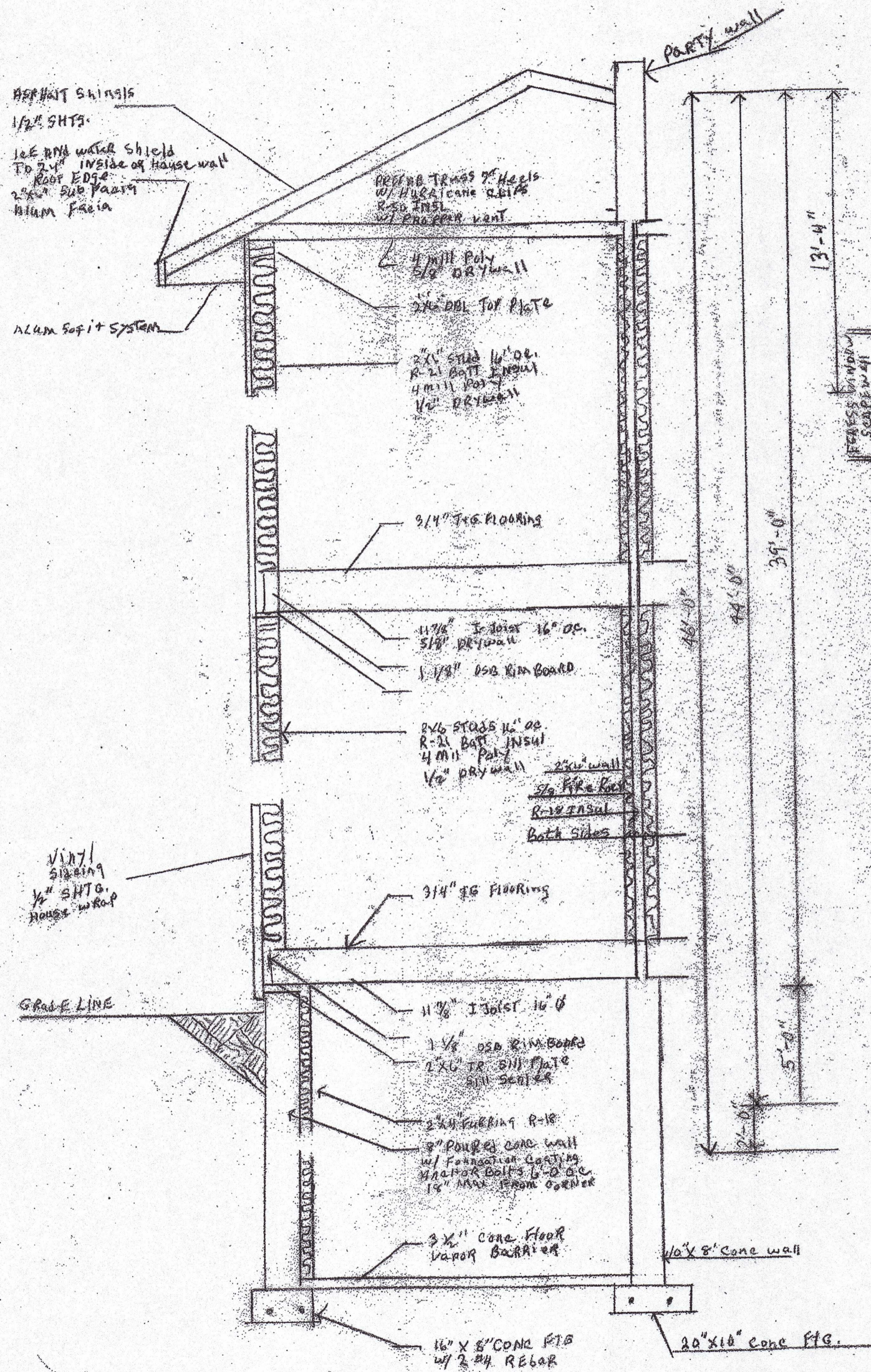
SECTION 1/2"
