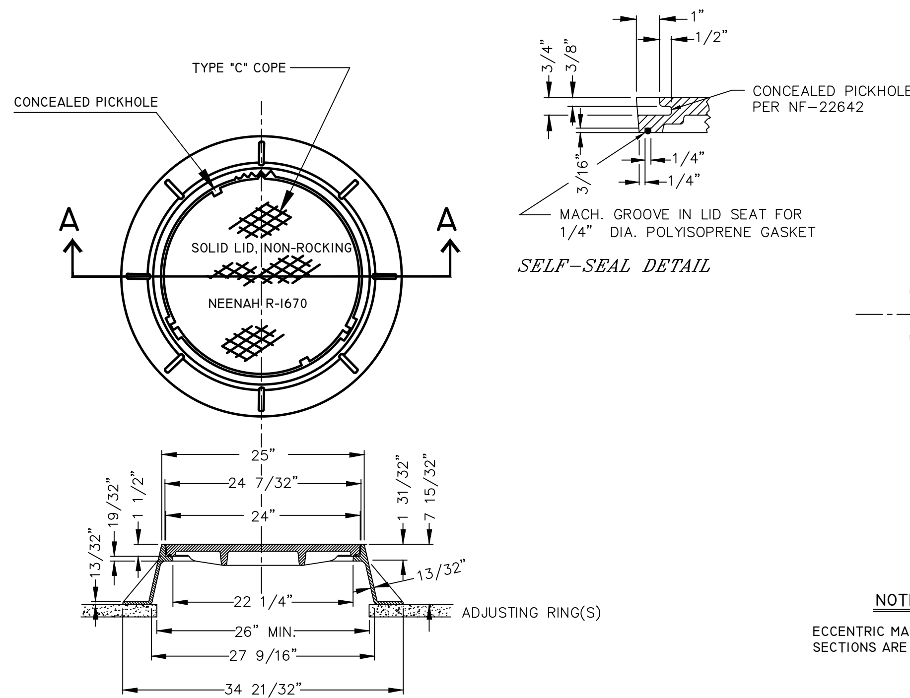
DETAIL OF MANHOLE FRAME & COVER
