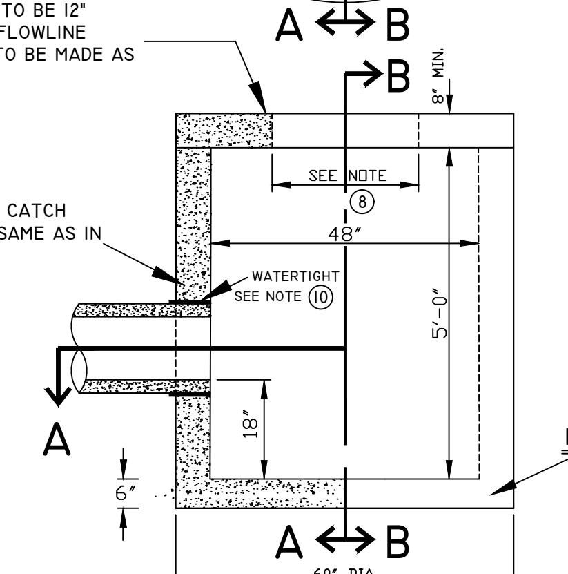
DETAIL OF TYPE "A" OR "B" CATCH BASIN
