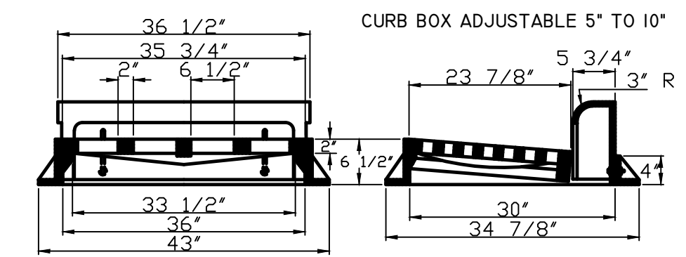
DETAILS OF TYPE "A" CATCH BASIN CASTING NEENAH R-3246-A OR APPROVED EQUAL
