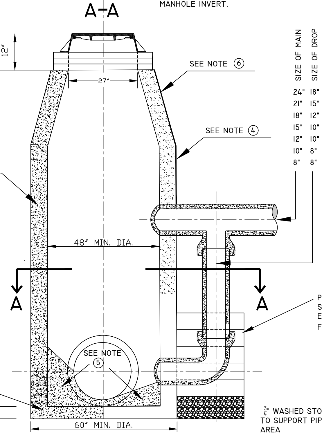
DETAILS OF DROP MANHOLE FOR 30" PIPE OR SMALLER
