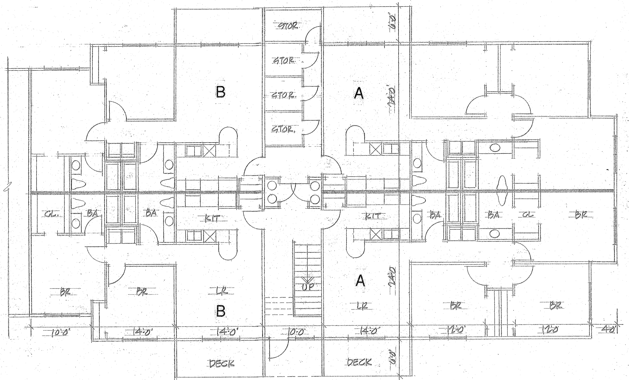
UNIT PLANS 1/8"=1'-0"
