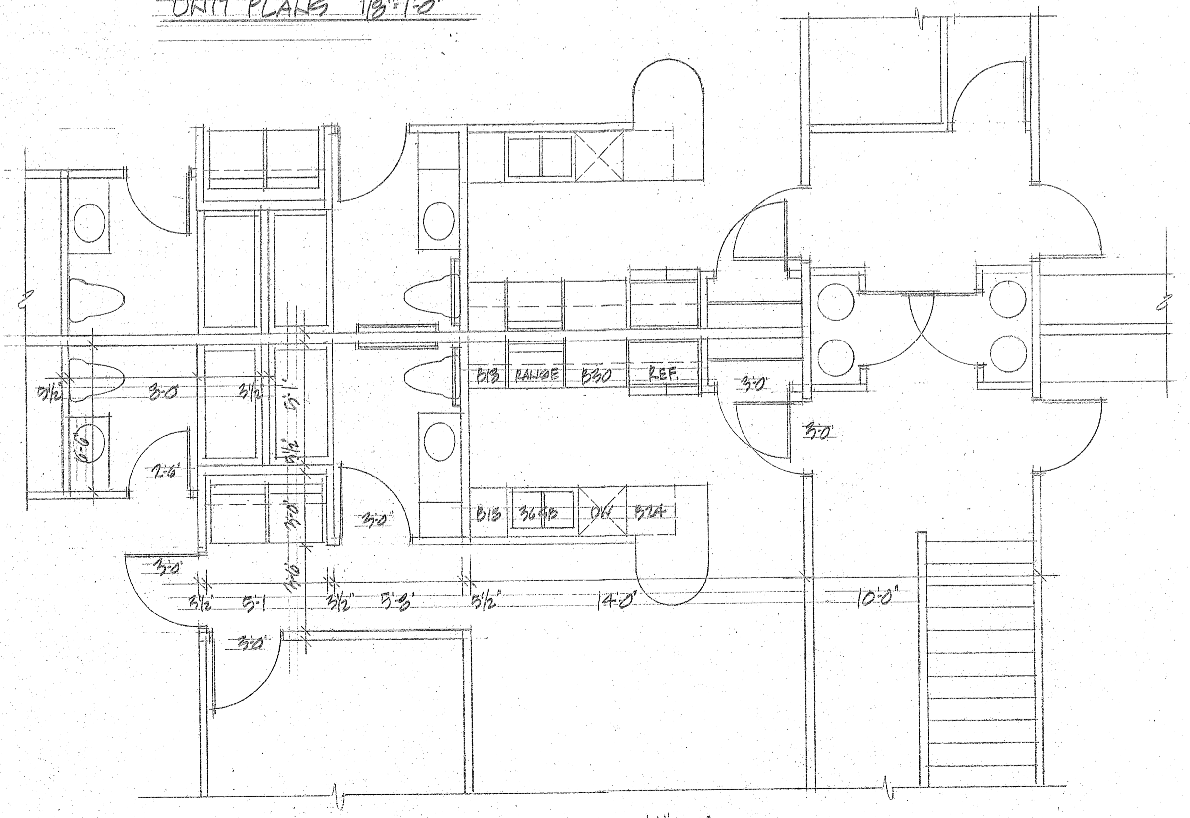
TYPICAL BATH & KITCHEN PLANS 1/4"=1'-0"
