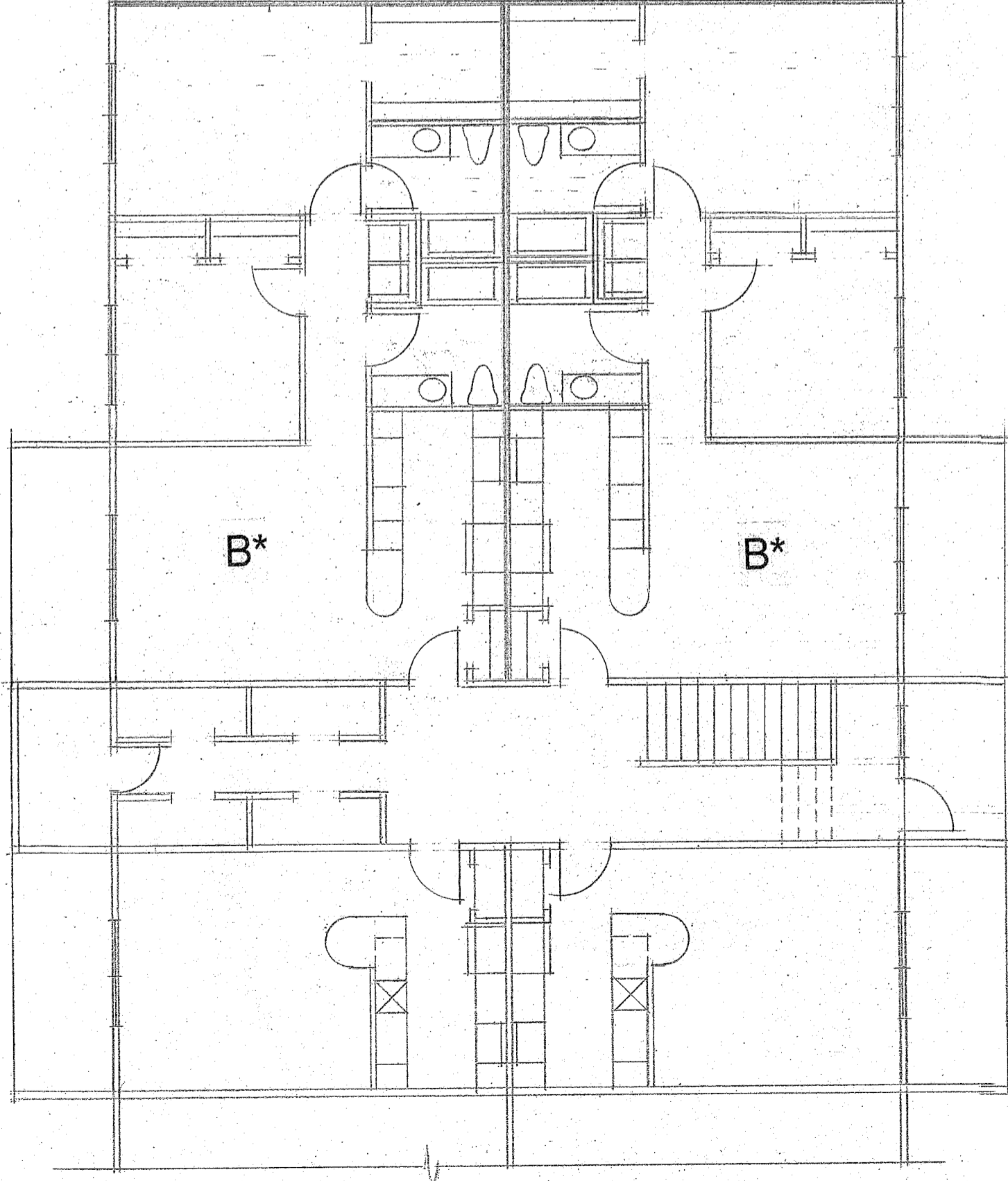
UNIT PLANS 1/8"=1'-0"
