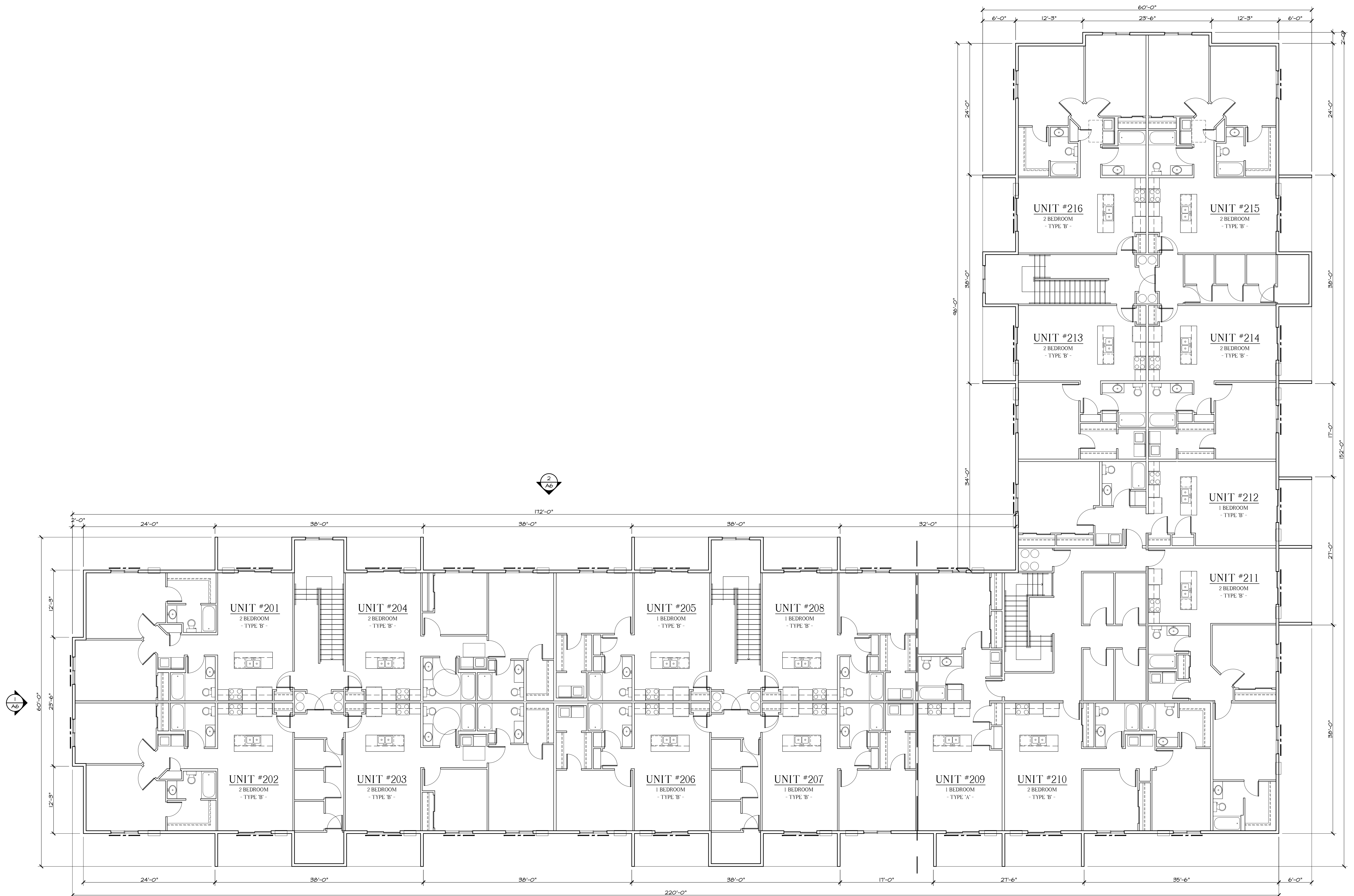
1 A2 SECOND FLOOR PLAN 1/8" = 1'-0"
