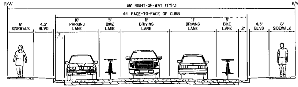
PROPOSED TYPICAL SECTION - JACKSON STREET 3RD STREET - 4TH STREET
