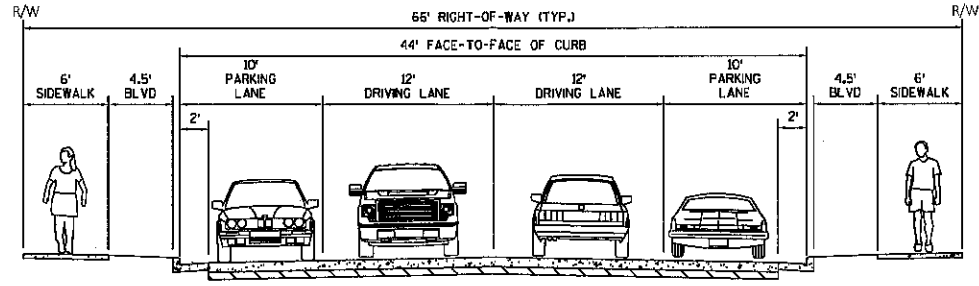
EXISTING/PROPOSED TYPICAL SECTION - JACKSON STREET 4TH STREET - 6TH STREET 8TH STREET - 11TH STREET 12TH STREET - 23RD STREET
