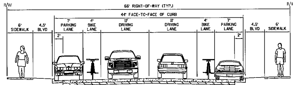
PROPOSED TYPICAL SECTION - JACKSON STREET 6TH STREET - 8TH STREET 11TH STREET - 12TH STREET
