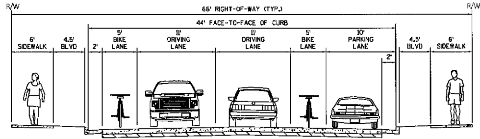
PROPOSED TYPICAL SECTION - JACKSON STREET 4TH STREET - 6TH STREET 8TH STREET - 11TH STREET 12TH STREET - 23RD STREET
