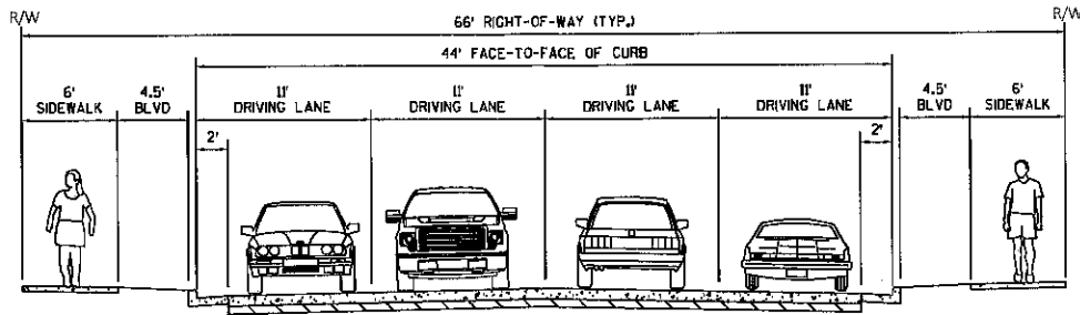
EXISTING/PROPOSED TYPICAL SECTION - JACKSON STREET 6TH STREET - 8TH STREET 11TH STREET - 12TH STREET
