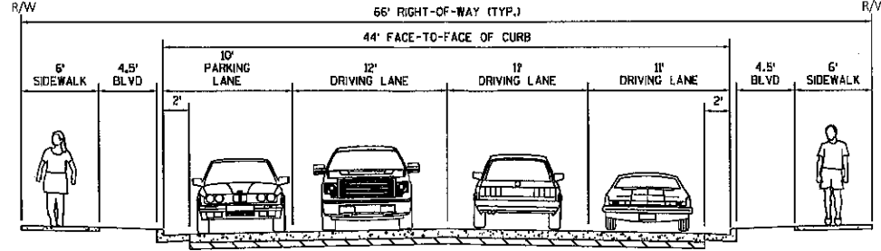
EXISTING/PROPOSED TYPICAL SECTION - JACKSON STREET 3RD STREET - 4TH STREET
