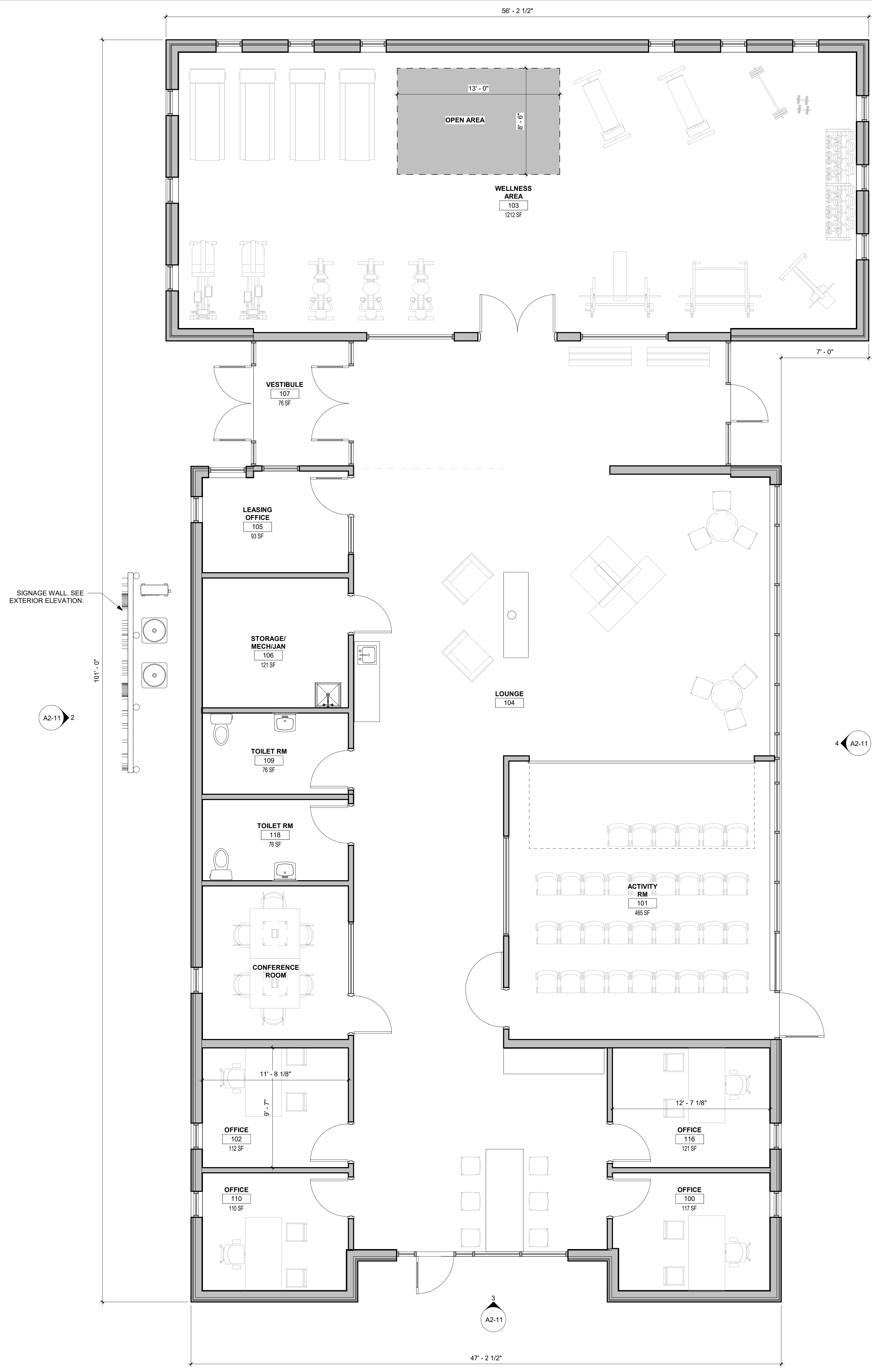
1 FLOOR PLAN 1/4" = 1'-0"
