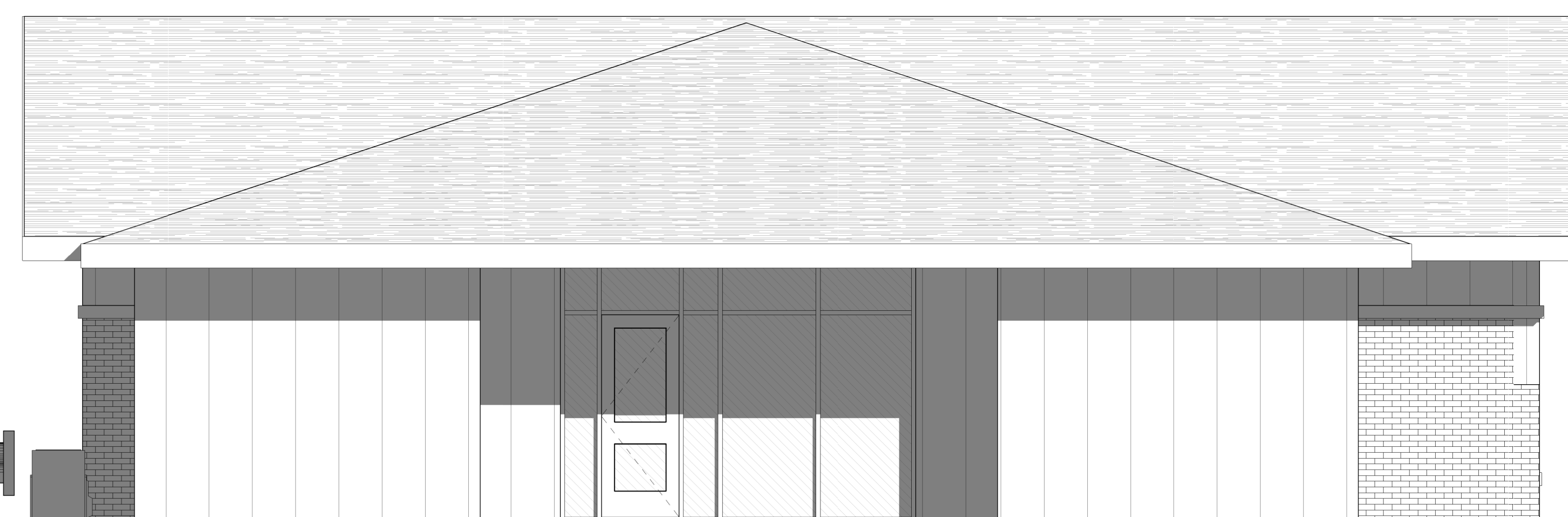
3 SOUTH ELEVATION 1/4" = 1'-0"
