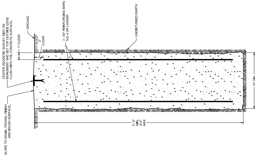
CAST-IN-PLACE CONCRETE MONUMENT
