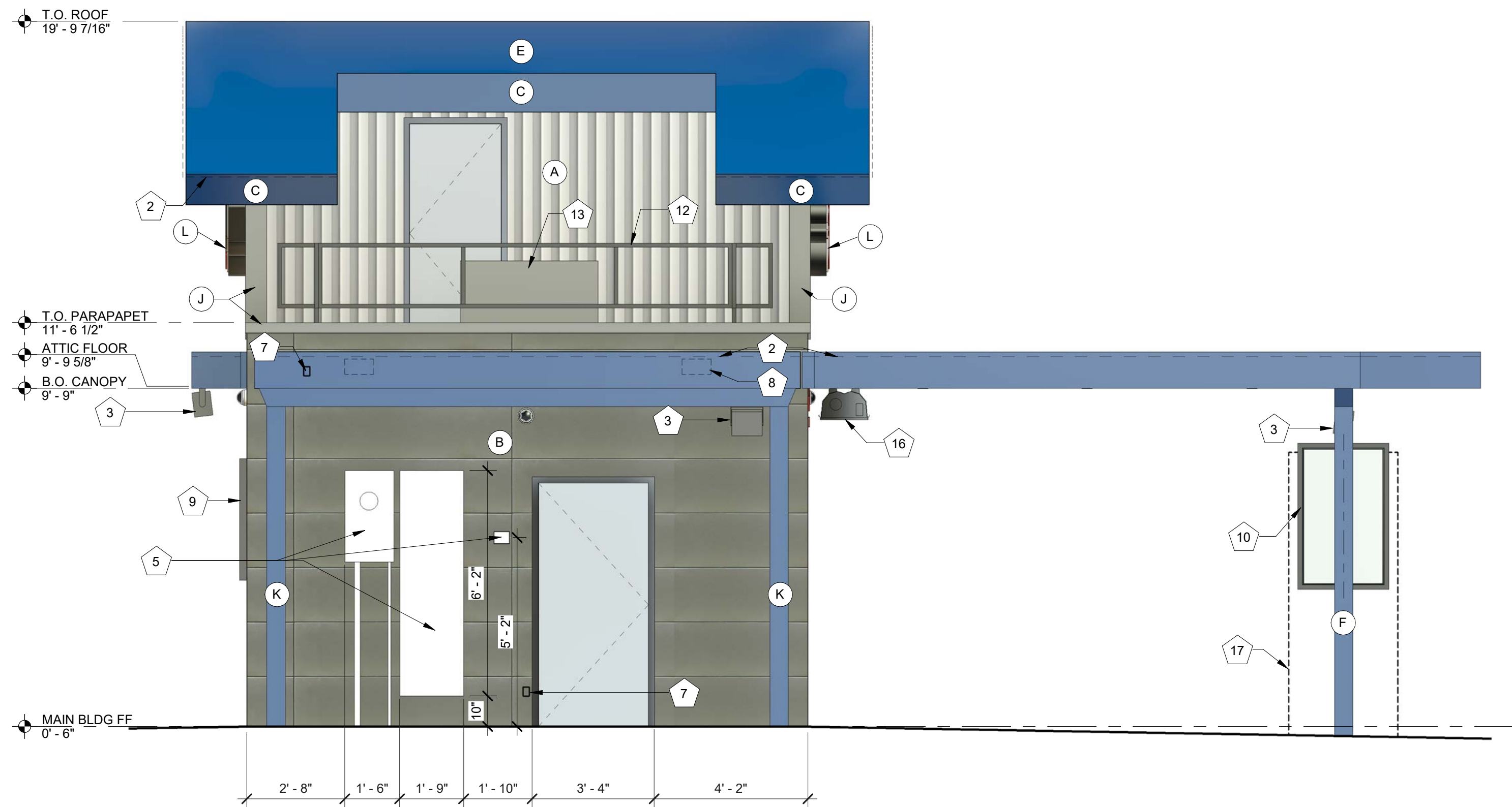
2 EXTERIOR ELEVATION - SOUTH
