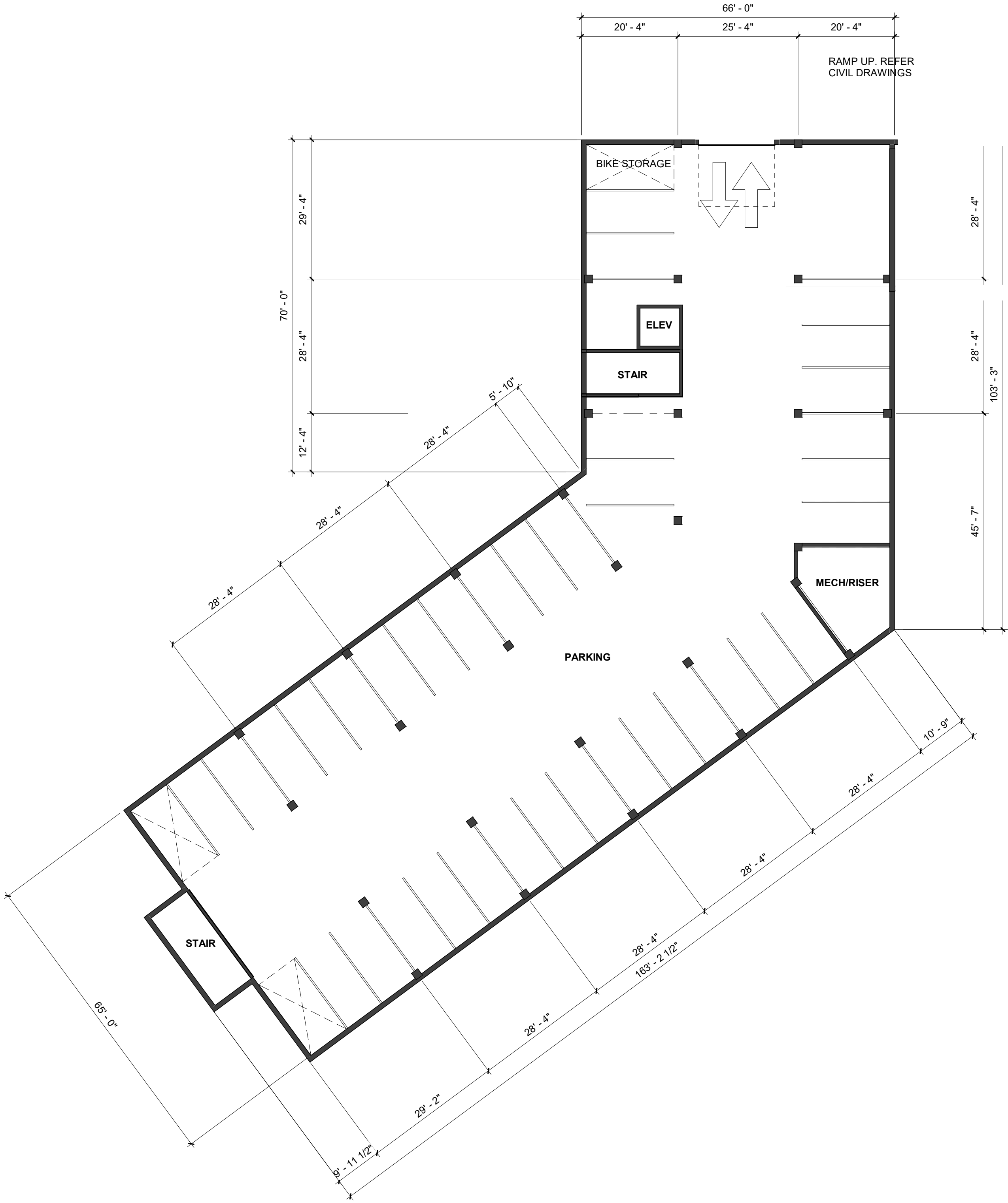
3 GARAGE LEVEL 1/16" = 1'-0"
