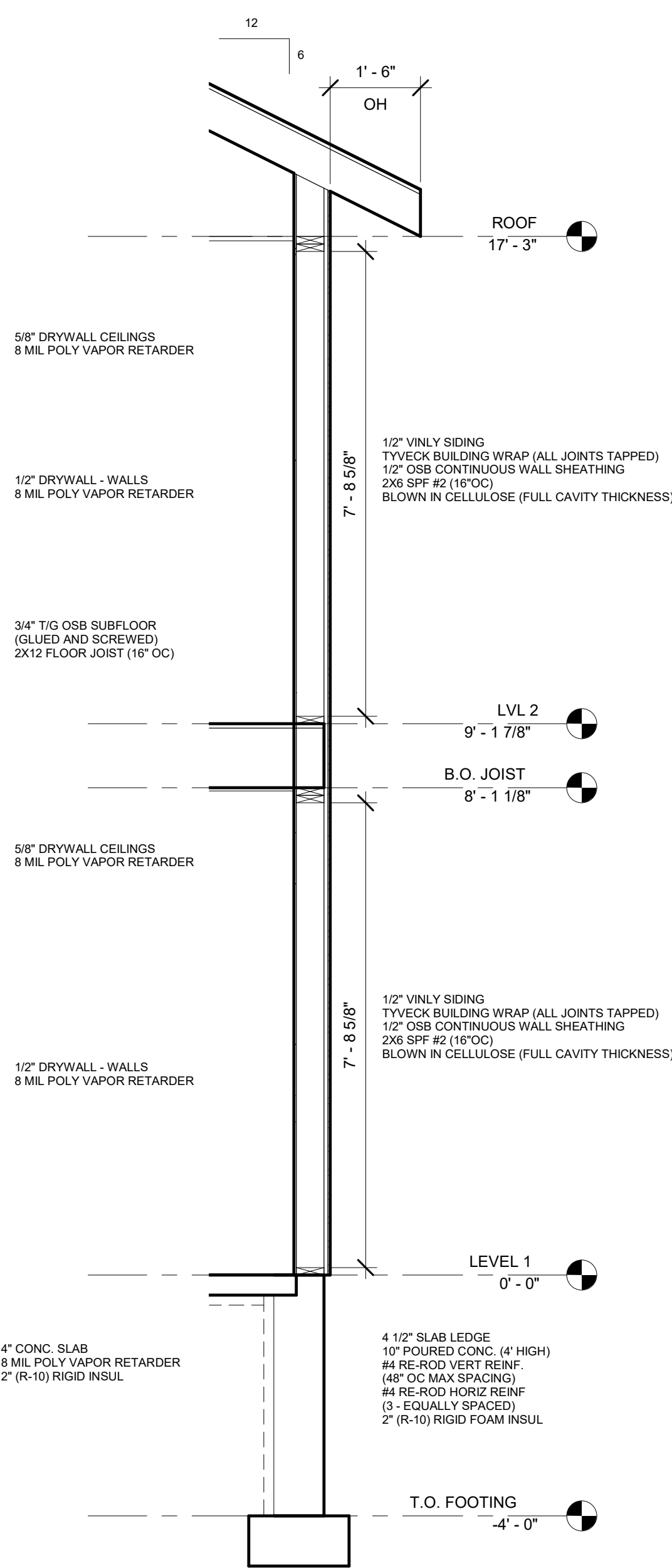
1 TYPICAL WALL SECTION 1/2" = 1'-0"
