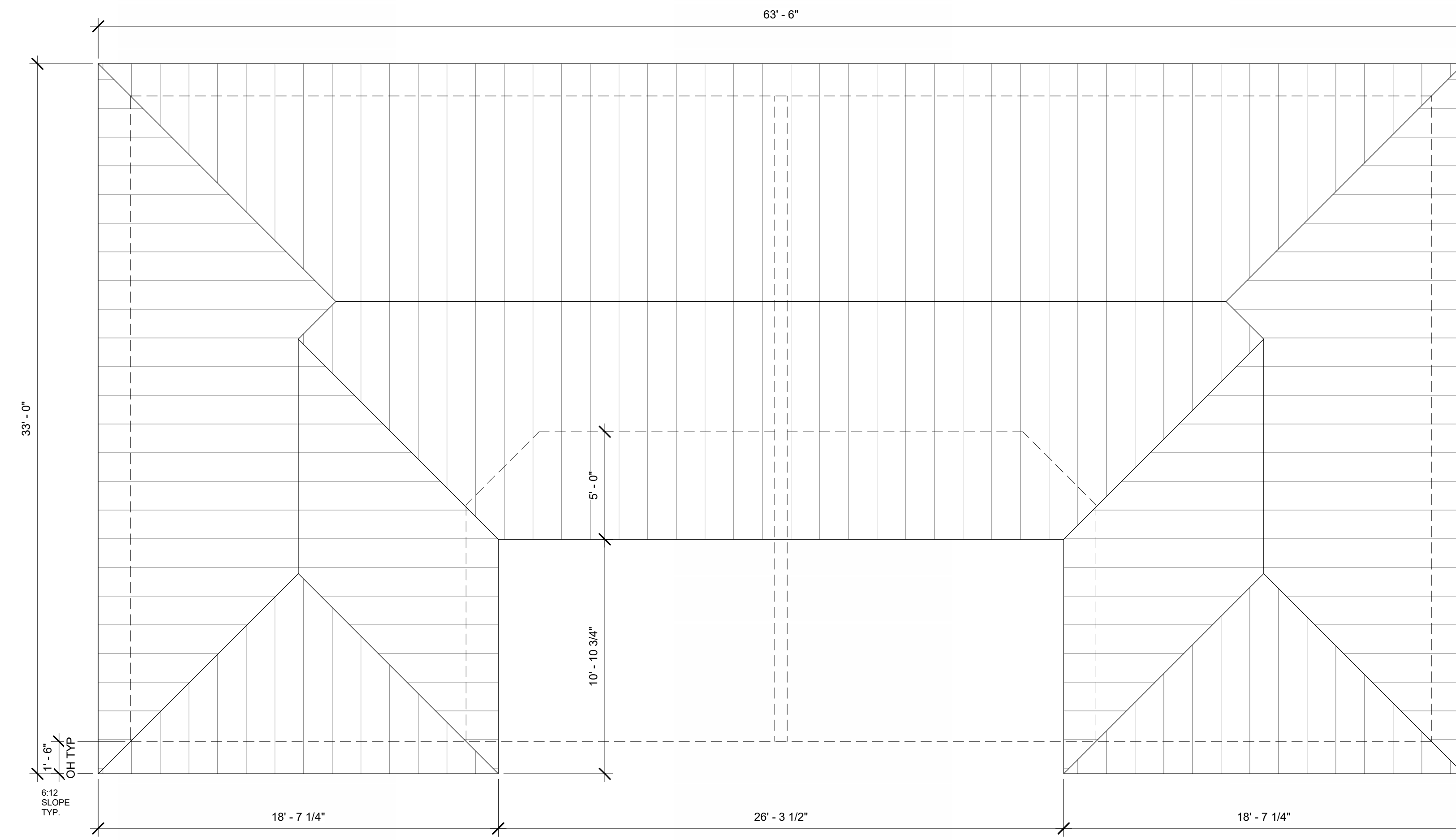
2 ROOF 1/4" = 1'-0"
