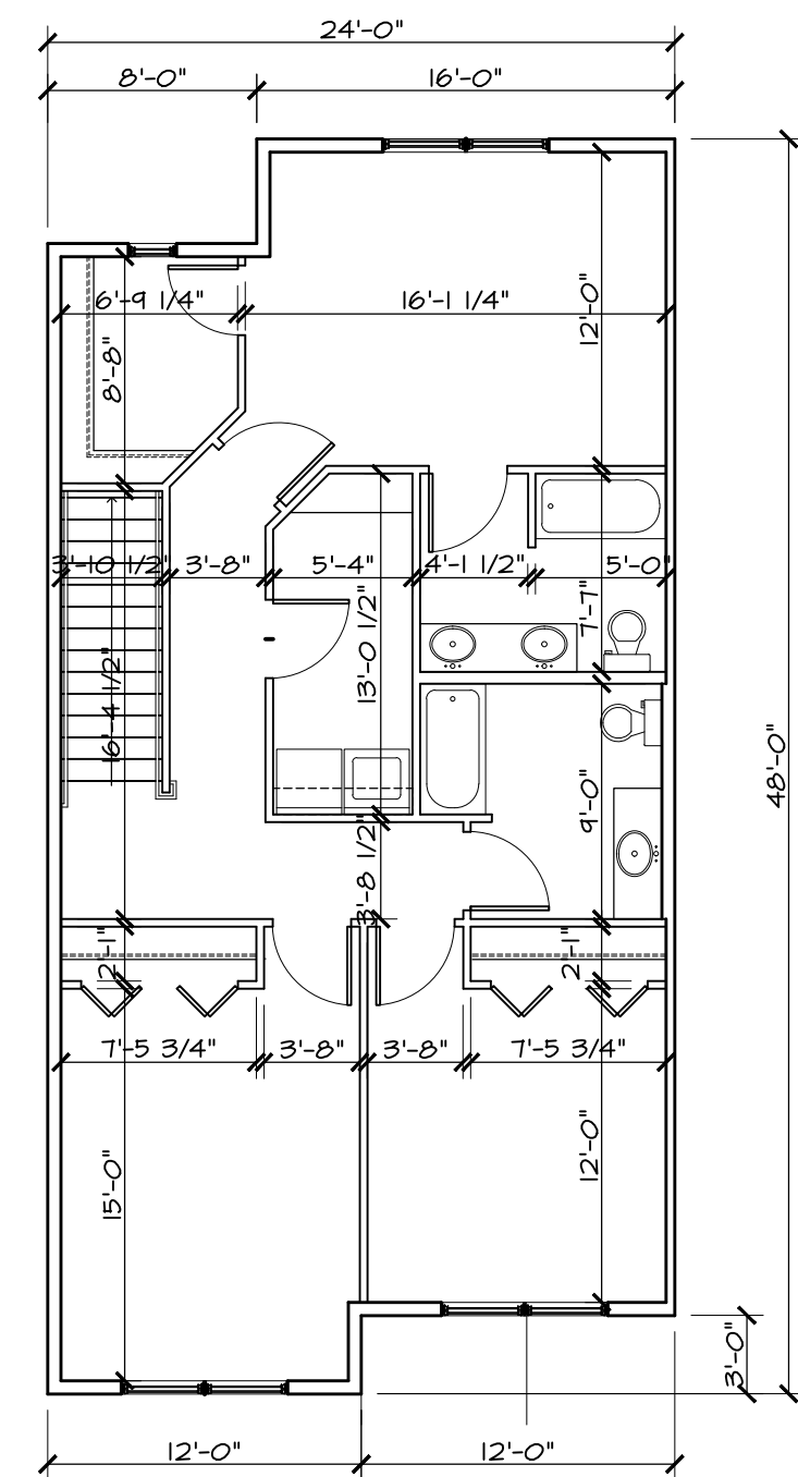
4 SECOND FLOOR 1/8" = 1'-0"
