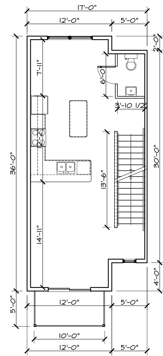
④ SECOND FLOOR A6 1/8" = 1'-0"
