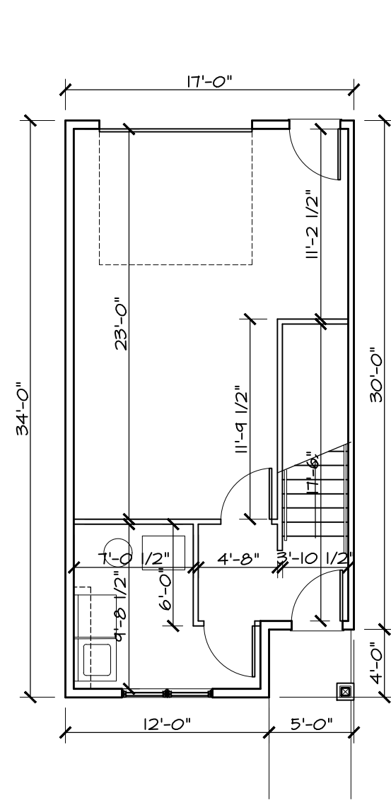
③ FIRST FLOOR A6 1/8" = 1'-0"
