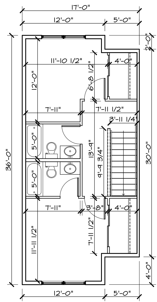
⑤ THIRD FLOOR A6 1/8" = 1'-0"
