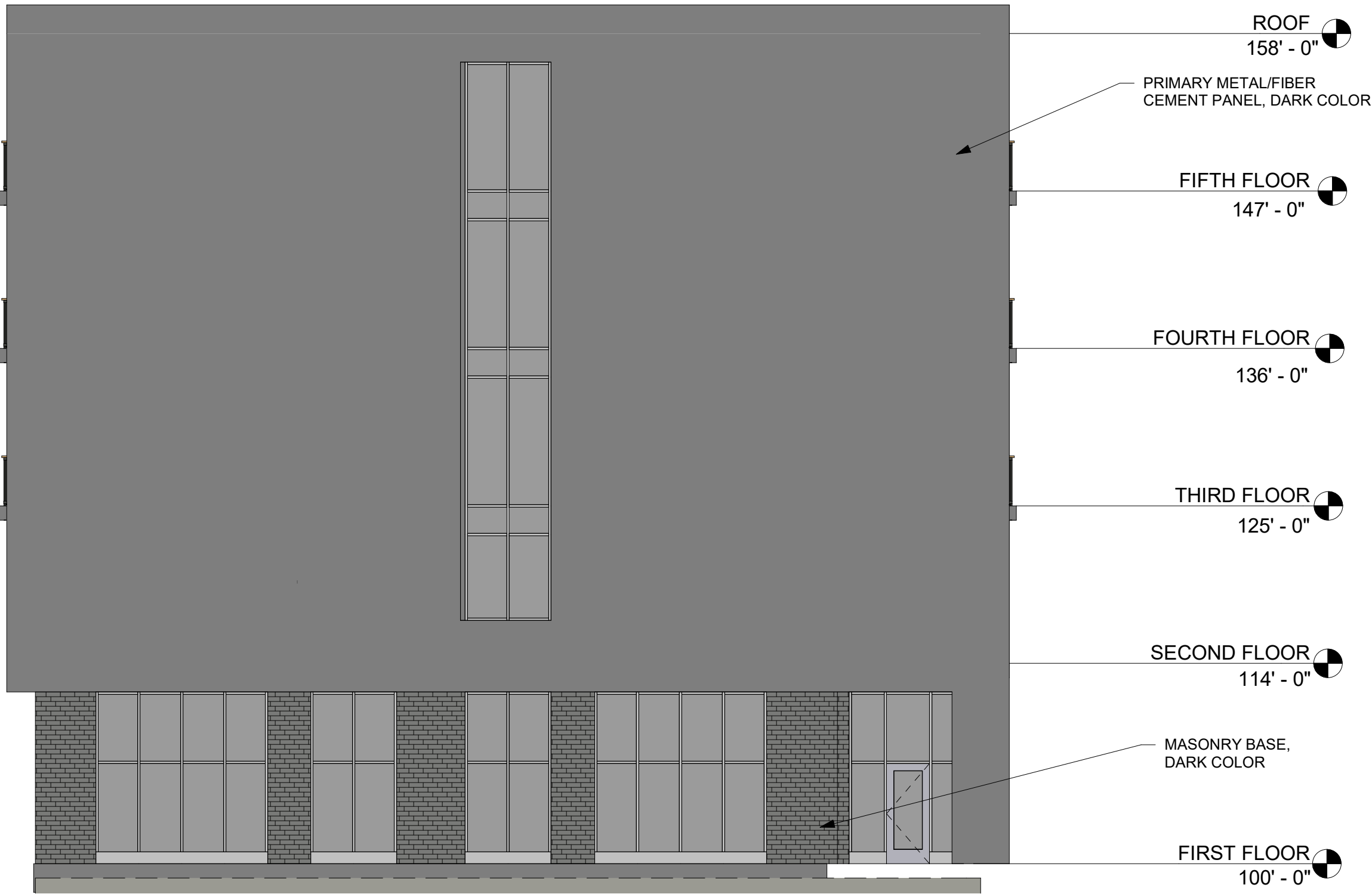
4 EAST BUILDING - SOUTH ELEVATION 1/8" = 1'-0"
