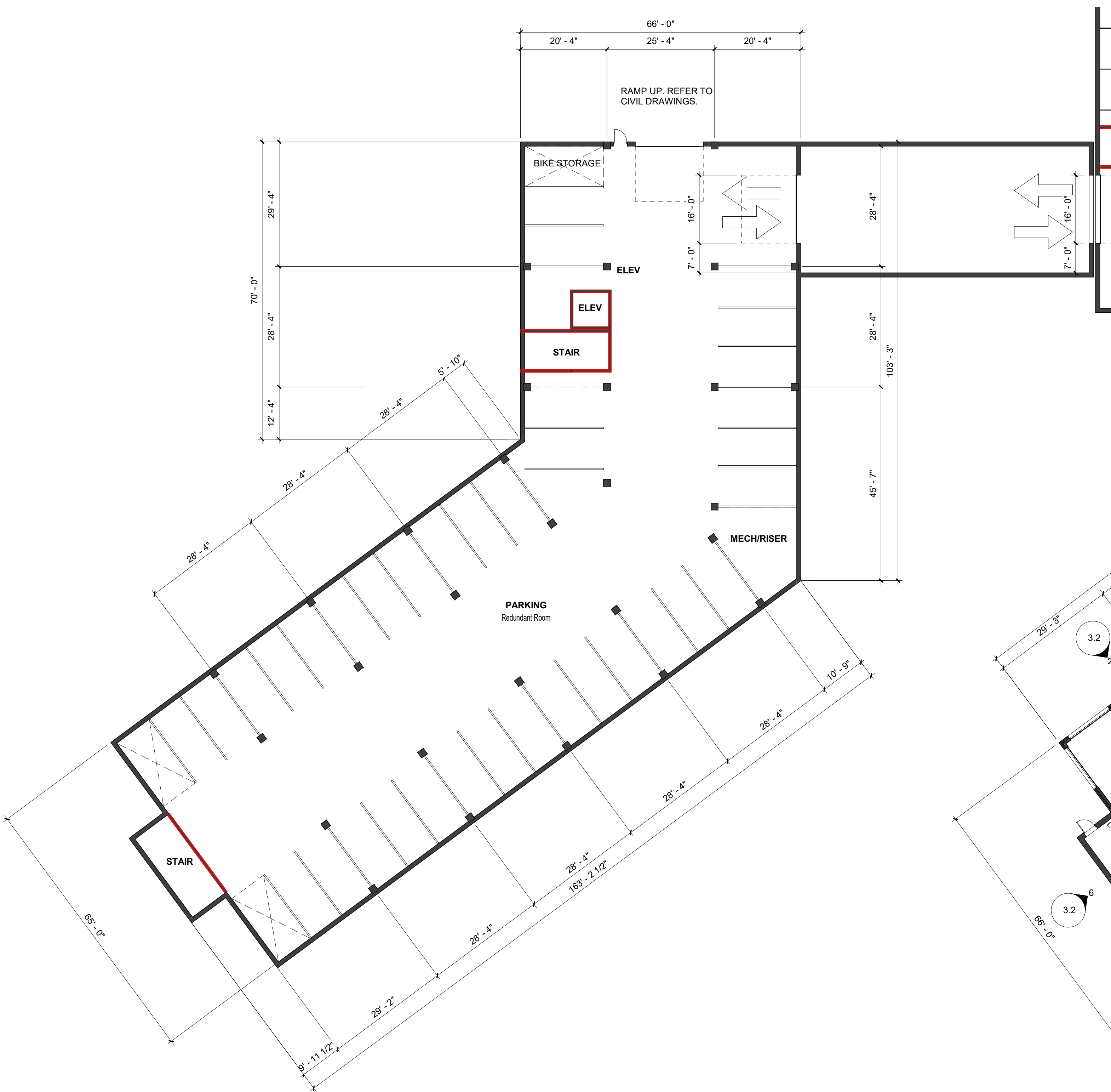
3 GARAGE LEVEL 1/16" = 1'-0"
