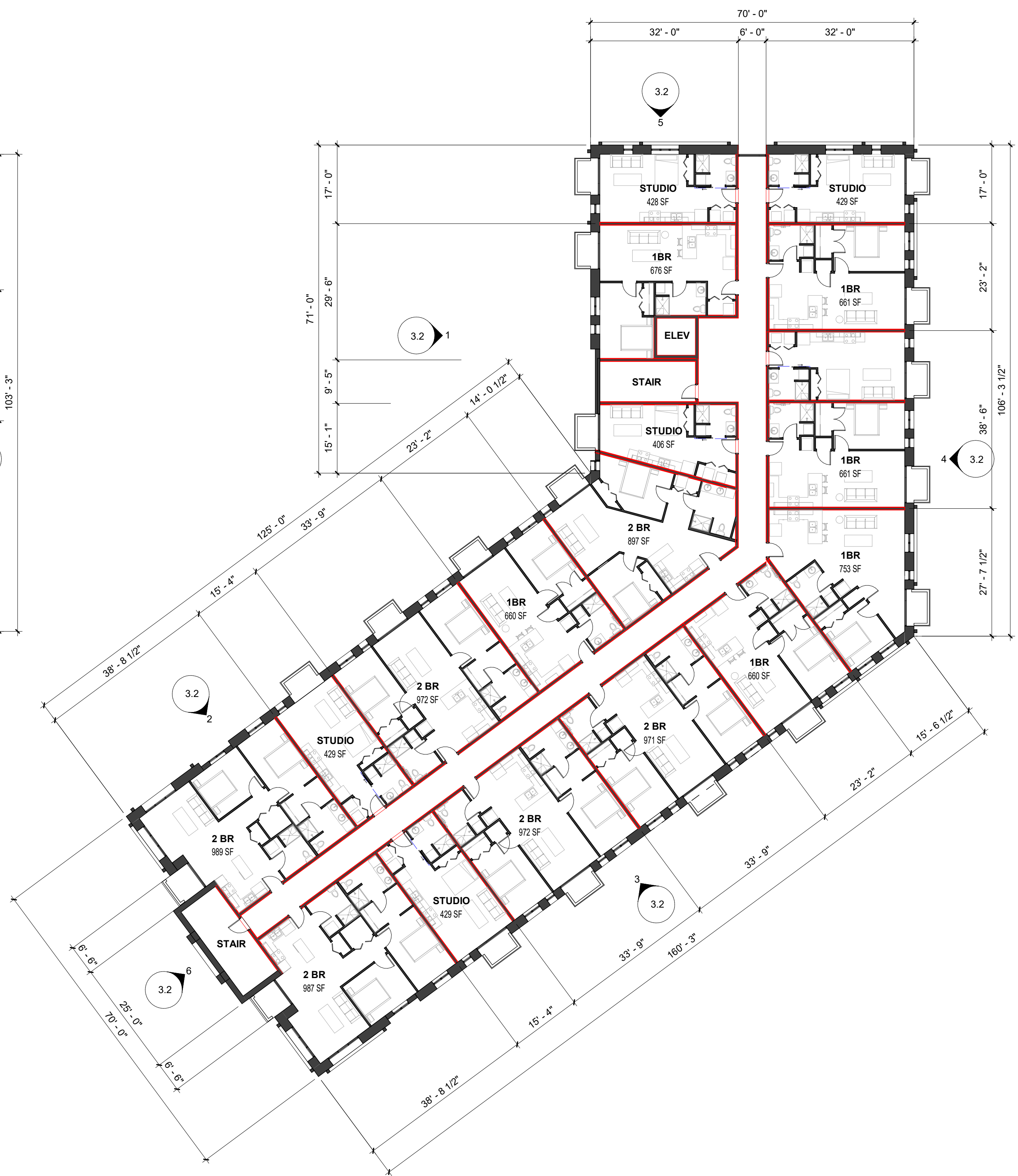
2 SECOND THRU FIFTH FLOOR PLAN 1/16" = 1'-0"
