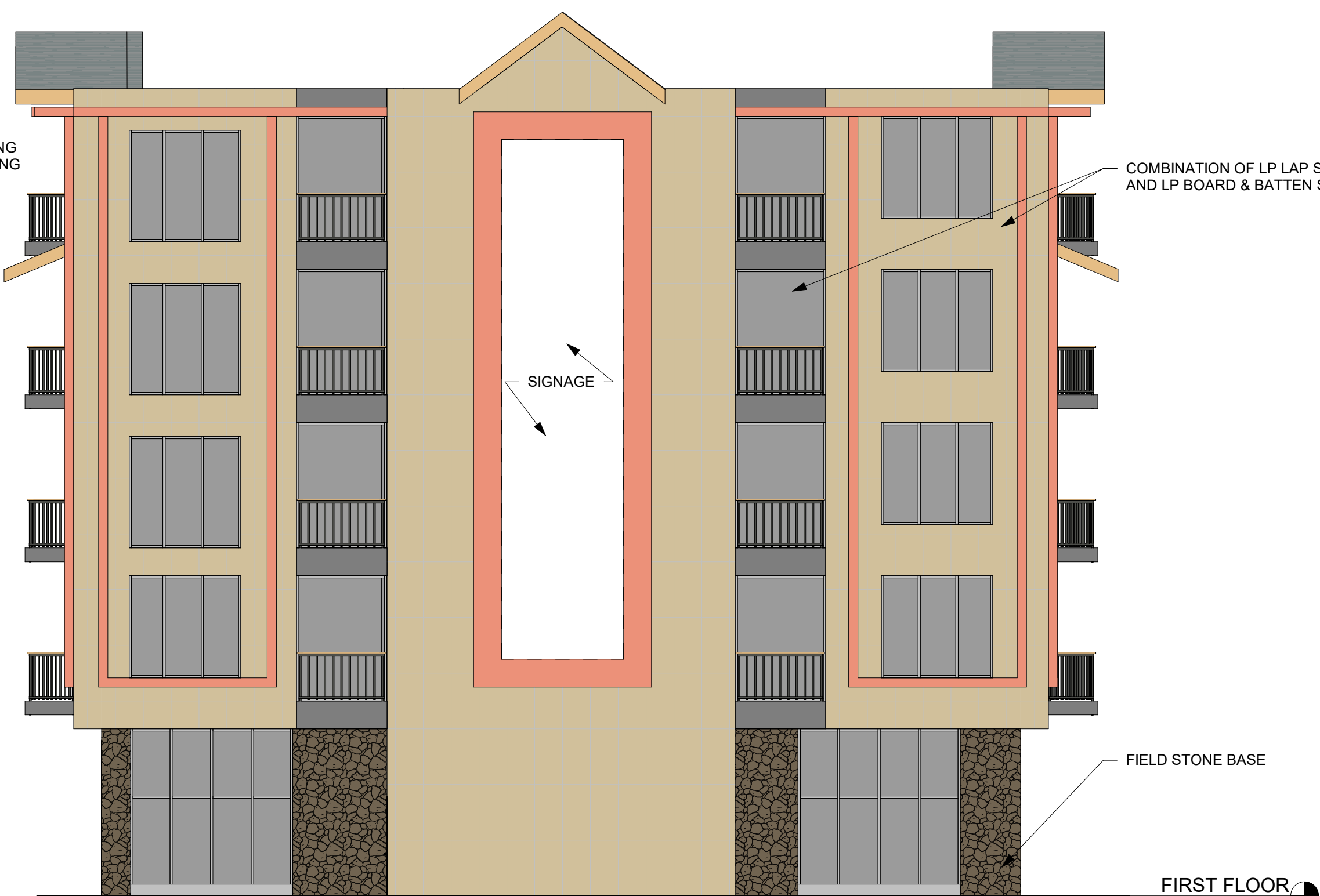
6 WEST BUILDING - SOUTH ELEV 1/8" = 1'-0"
