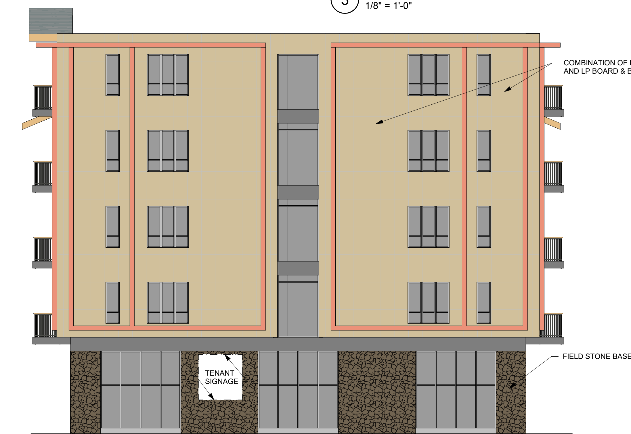
5 WEST BUILDING - NORTH ELEVATION 1/8" = 1'-0"
